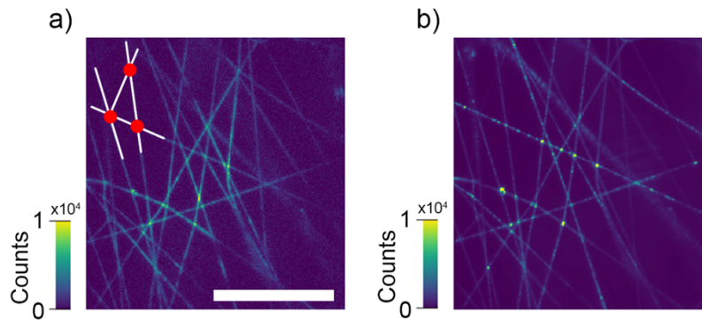
Fig. 12. Nanophotonic RL on a graph [90]. Far-field images of fluorescence (a) and lasing (b) from a network of free-standing subwavelength electrospun polymer nanofibres embedded with dye. Scale bar is 100 \mu\text{m} .
