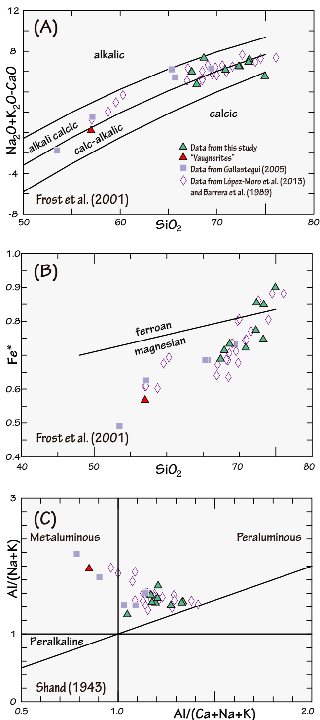
Figure 3. Geochemical features of the early Carboniferous suite (ECS) granitoids. (A) SiO 2 versus Na 2 O + K 2 O - CaO diagram of Frost et al. (2001). (B) SiO 2 versus FeO total /(FeO total + MgO) diagram (Frost et al., 2001). (C) A/CNK (molar ratio of Al 2 O 3 /CaO + Na 2 O + K 2 O) versus A/NK diagram (Shand, 1943).
