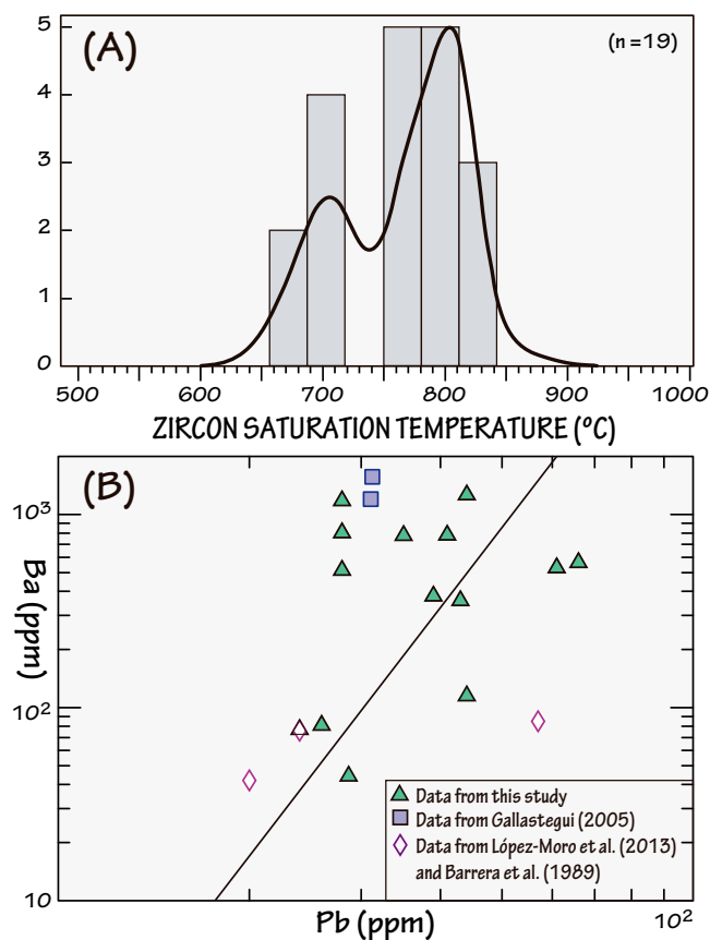
Figure 9. (A) KDE (kernel density estimation) plot of the zircon saturation temperature (calculated according to Watson and Harrison, 1983) for the early Carboniferous suite (ECS) granitoids (see main text for details). (B) Pb versus Ba diagram (Finger and Schiller, 2012) for the ECS granitoids (see main text for details).
