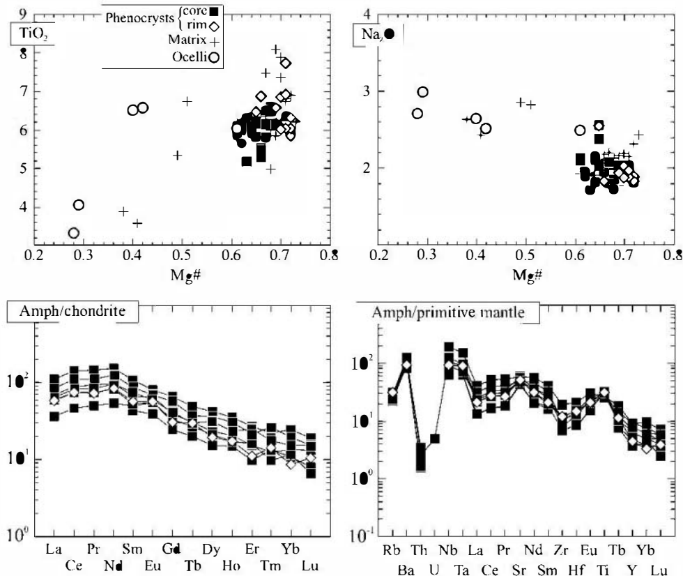
Fig. 3 Major and trace element composition of amphibole from the SCS alkaline basic dykes. The normalising values of chondrite and primitive mantle are after Sun and McDonough (1989) and McDonough and Sun (1995), respectively
