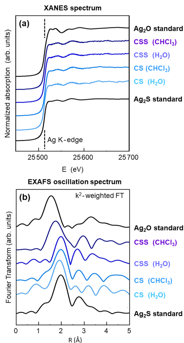
Fig. 4 (a) XANES spectra at the Ag K-edge of CS and CSS NCs solutions in CHCl 3 and water, compared with Ag 2 S and Ag 2 O standards. (b) Fourier transform (FT) of the k^2 -weighted EXAFS oscillations, for all NCs systems shown in (a).
