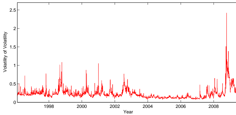
FIGURE 9. S&P500 Estimated Volatility of Realized Volatility.
