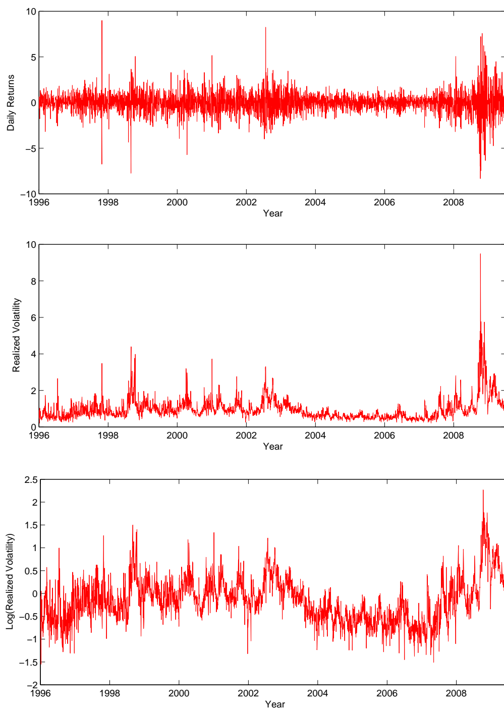
FIGURE 7. Time Series of returns (top), realized volatility (middle) and log realized volatility (bottom) for the S&P 500 index.
