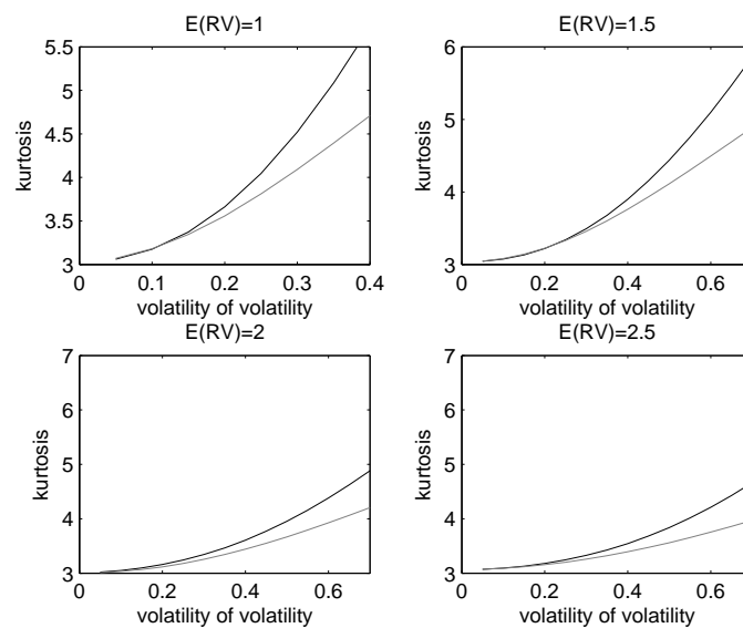
FIGURE 1. Kurtosis of the simulated distribution under the assumption that shocks to realized have the NIG (upper line) and normal distributions.
