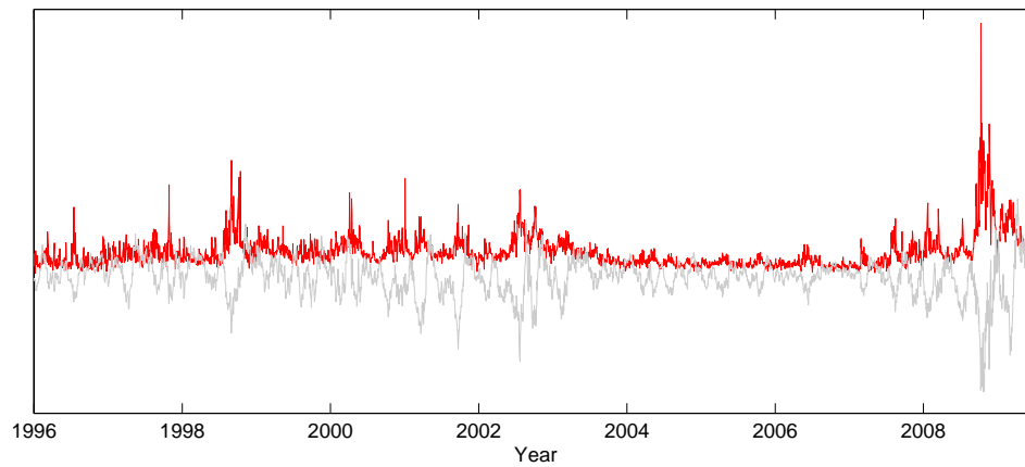
FIGURE 8. Realized Volatility (top) and Monthly Returns (bottom) for the S&P 500 index.
