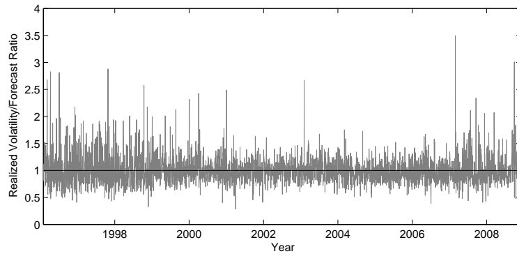
FIGURE 3. In-Sample Percentage Errors for the HAR model with leverage effects.
