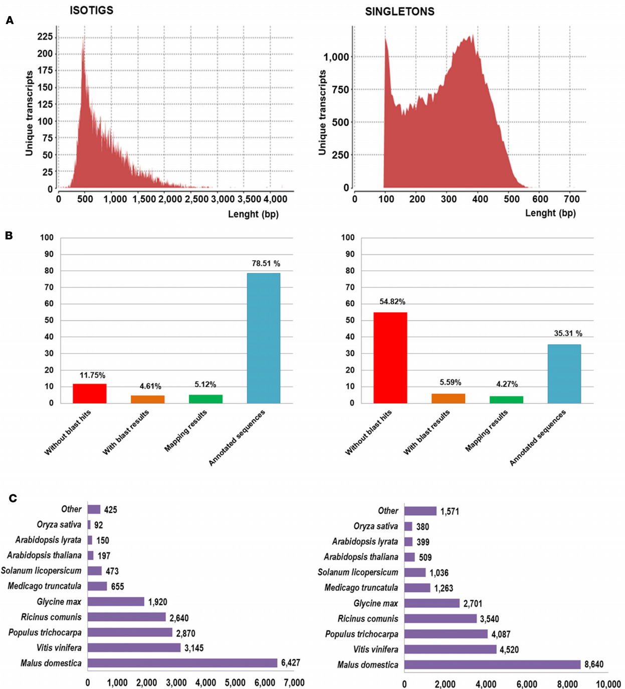
FIGURE 1 | Sequence length and blast results distribution for isotigs and singletons. (A) Sequence length distributions for unique transcript identified after assembly (B) Proportion of Ulmus minor transcript without homology with plant proteins (without blast hits), with homology but no associated function
