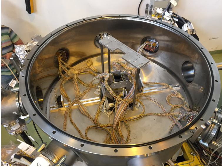
Figure 3.6: Arrangement of the IS619 setup inside the SEC chamber in August 2017.
