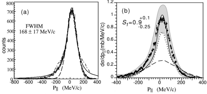
Figure 1.11: (a) Longitudinal momentum distribution from ^{17}\text{Ne} to ^{15}\text{O} with a Be target at 66 MeV/u. (b) Comparison assuming a model of ^{15}\text{O} core plus two uncorrelated protons. Solid line shows the result for a pure s-wave configuration ( S_1=1 ) and long-dashed line for a pure d-wave configuration ( S_1=0 ). A combination of these two extreme cases is set to reproduce the data. Picture taken from [28].
