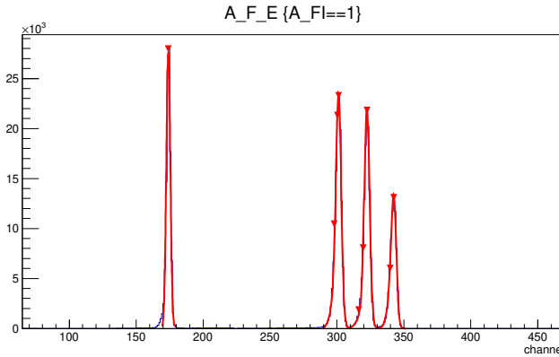
Figure 5.1: Gaussian fits to the 4 emitters in the alpha source used for calibration. Spectrum of the first front strip of detector A . Centroids of the fits are remarked with a triangle. Notice that only the first 475 channels of the spectrum are shown.
