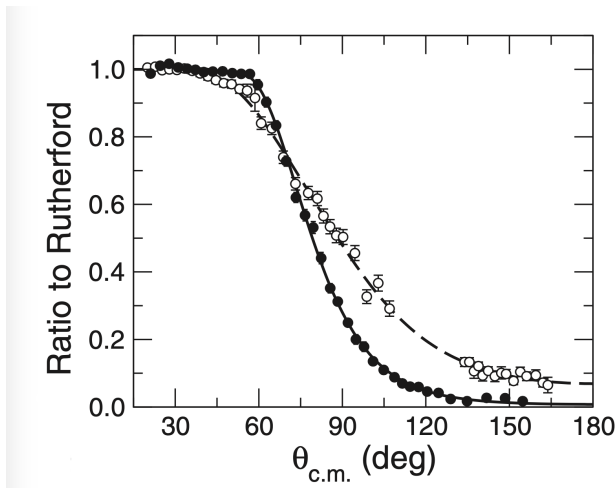
Figure 1.6: Angular distribution of the elastic cross for ^6\text{He} (empty circles) and ^8\text{He} (filled circles) on ^{208}\text{Pb} near the Coulomb barrier. Picture from [17].
