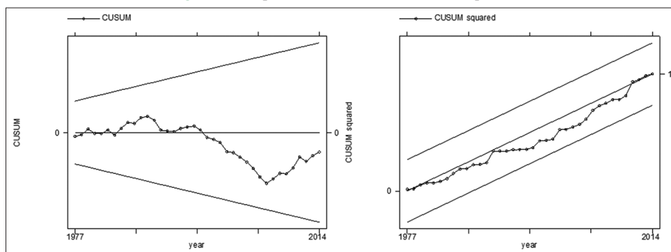
Figure 3: Graphs of CUSUM and CUSUM squared
