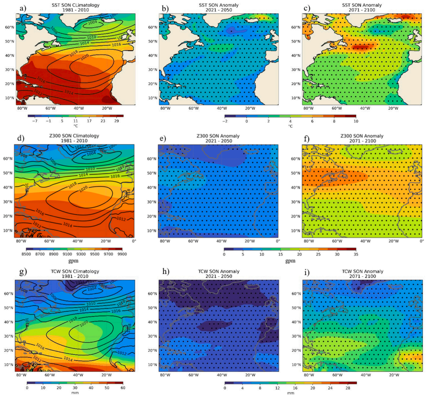
Fig. 1. Seasonal climatological values in SON for the 1981–2010 period of a) SST (°C) and MSLP (hPa; black contours), d) Z300 (gpm) and MSLP (hPa; black contours). Seasonal anomaly values in SON with respect to the climatology of SST (°C) for the b) near and c) far future period; of Z300 (m) for the e) near and f) far future period; of TCW (mm) for the h) near and i) far future period. Black dots indicate where the anomalies computed are statistically significant (Mann – Whitney U test; \alpha = 0.05 ).
