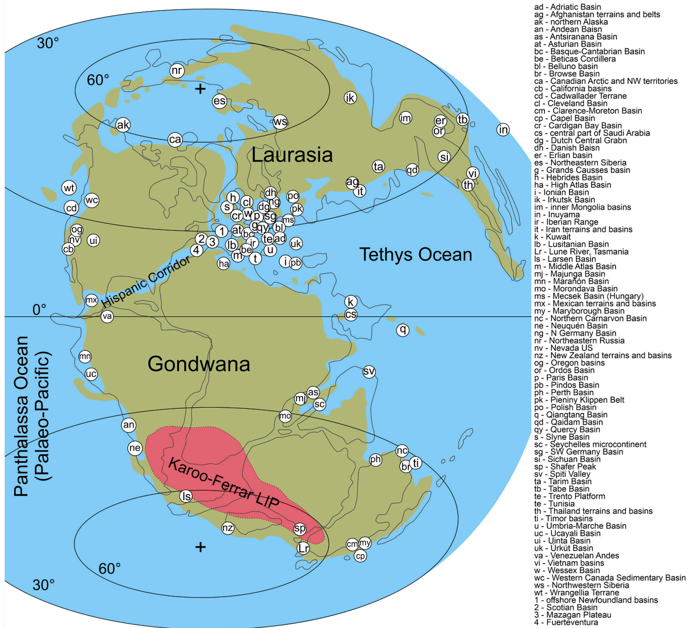
Fig. 1. Base map with Early Jurassic continent positions and locations of basins and localities with known Lower Jurassic sediments (modified from Damborenea (2002) and references therein). For simplicity, the West Netherlands Basin, Southern Beaujolais, Sub-Briançonnais Basin, Northern Calcareous Alps, and Midlands shelf are not represented here.
