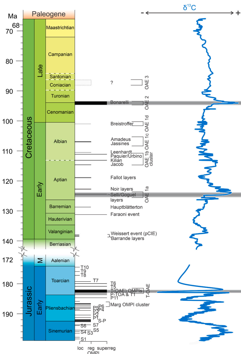
Fig. 5. Mesozoic OAEs and comparison with the Early Jurassic OMPIs record (the grey bars correspond to the main Jurassic–Cretaceous OAEs). The Sinemurian–Pliensbachian record was created using the time scale and \delta^{13}\text{C} from the reference Mochras core, Cardigan Bay Basin, UK (Storm et al., 2020). The Toarcian and Cretaceous time scale (Ogg et al., 2016) and \delta^{13}\text{C} record (Herrle et al., 2004; Reichelt, 2005; Föllmi et al., 2006; Jarvis et al., 2006; Hesselbo et al., 2007; Voigt et al., 2012; Martinez et al., 2015; Xu et al., 2018) were generated using TSCreator software (PUBLIC7.4_windows10_latest_06September2019). Cretaceous OAEs are from Arthur et al. (1990); Leckie et al. (2002); Bodin et al. (2007); Mutterlose et al. (2009); Jenkyns (2010); Westermann et al. (2010); Föllmi et al. (2012); Herrle et al. (2015).
