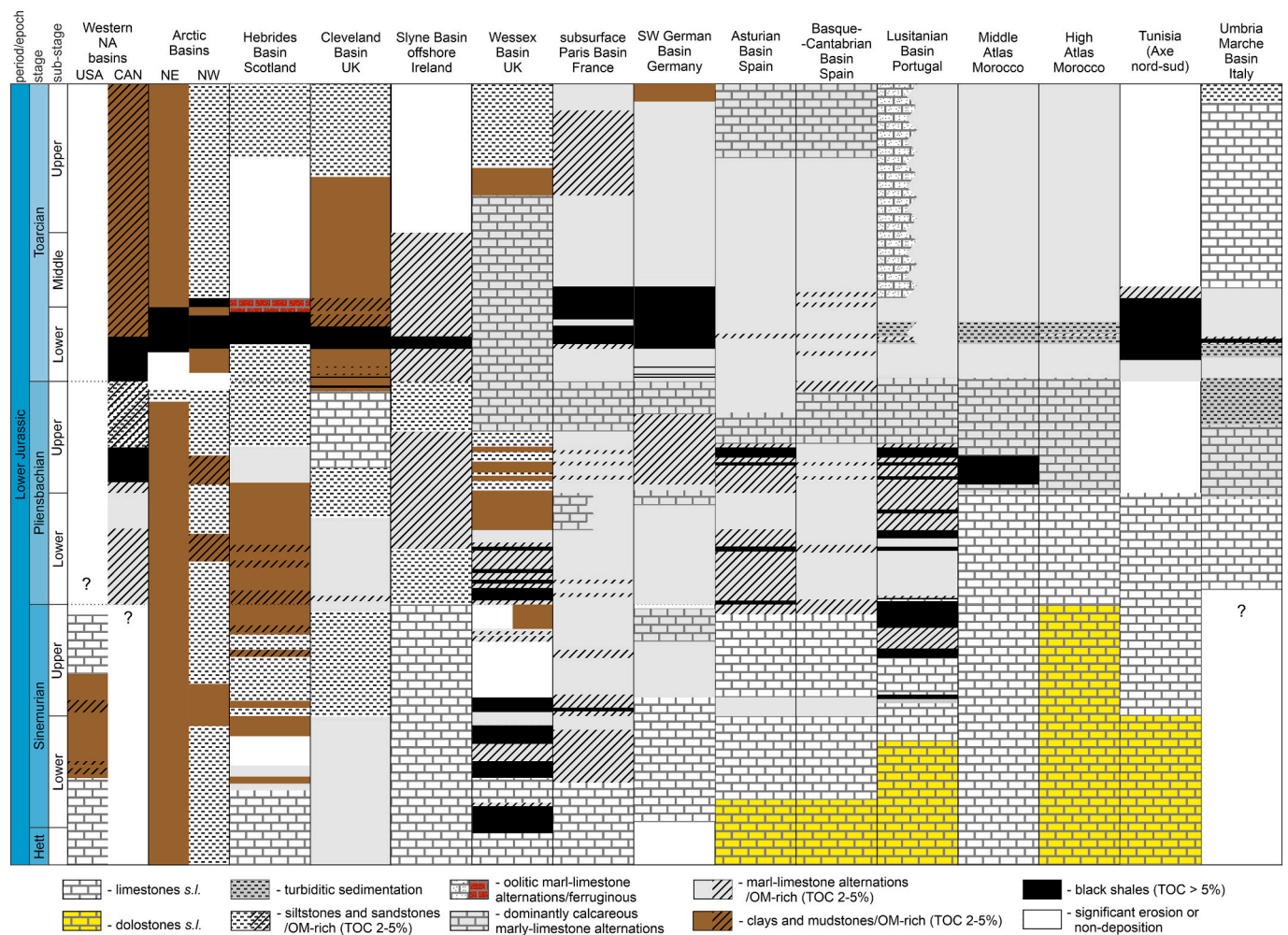
Fig. 2. General temporal and paleogeographical trends of Lower Jurassic organic-rich sedimentary successions. Western North America (NA) basins : Stratigraphy - (Asgar-Deen et al., 2003); Organic-rich facies - (Caruthers et al., 2011; Porter et al., 2014b; Porter et al., 2014a; Them et al., 2017); Arctic Basins : Stratigraphy - (Shurygin et al., 2011); Organic-rich facies - NE (Suan et al., 2011); NW (Kontorovich et al., 1997); Hebrides Basin (Scotland) : Stratigraphy - (Hesselbo et al., 1998; Hesselbo and Coe, 2000; Morton, 2004); Organic-rich facies - (Thrasher, 1992; Trueblood, 1992; Scotchman, 2001); Cleveland Basin (UK) : Stratigraphy - (Hesselbo et al., 2000b; Simms et al., 2004; Korte and Hesselbo, 2011); Organic-rich facies - (Jenkyns and Clayton, 1997; Scotchman, 2001; Kemp et al., 2005; Wignall et al., 2005; McArthur et al., 2008; Littler et al., 2010; Caswell and Coe, 2012; Salem, 2013; Porter et al., 2014a; Song et al., 2015); Slyne Basin (offshore Ireland) : Stratigraphy - (Dancer et al., 2005); Organic-rich facies - (Trueblood, 1992; Scotchman, 2001; Silva et al., 2017); Wessex Basin (UK) : Stratigraphy - (Simms, 2004; Gallois, 2008; Jenkyns and Weedon, 2013); Organic-rich facies - (Jenkyns and Clayton, 1997; Weedon and Jenkyns, 1999; Scotchman, 2001; Deconinck et al., 2003; Ruhl et al., 2010; Jenkyns and Weedon, 2013; Price et al., 2016; Xu et al., 2017a); Paris Basin (France) : Stratigraphy - (Mouterde et al., 1980); Organic-rich facies - (Bessereau et al., 1995; van Breugel et al., 2006; Hermoso et al., 2012, 2013, 2014; Lézin et al., 2013; Song et al., 2014); SW Germany : Stratigraphy - (Menning and Hendrich, 2002; Pieńkowski et al., 2008; Feist-Burkhardt and Pross, 2010); Organic-rich facies - (Röhl et al., 2001; Schmid-Röhl et al., 2002; Röhl and Schmid-Röhl, 2005); data in (McArthur et al., 2008); (Song et al., 2015); Asturian Basin (Spain) : Stratigraphy - (Aurell et al., 2003; Comas-Rengifo and Goy, 2010); Organic-rich facies - (Borrego et al., 1996; Gómez et al., 2008, 2016a; Gómez and Goy, 2011); this study; Basque-Cantabrian Basin (Spain) : Stratigraphy - (Aurell et al., 2003); Organic-rich facies - (Quesada et al., 1997, 2005; Gómez and Goy, 2011); Lusitanian Basin (Portugal) : Stratigraphy - (Duarte and Soares, 2002; Duarte et al., 2010, 2014; Silva et al., 2011, 2015); Organic-rich facies - (de Oliveira et al., 2006; Duarte et al., 2010, 2012; Silva et al., 2010, 2012; Silva et al., 2011, 2012; Poças Ribeiro et al., 2013; Silva, 2015; Silva and Duarte, 2015); this study; Middle Atlas (Morocco) Stratigraphy - (Sadki et al., 2014); Organic-rich facies - (Rachidi et al., 2009; Sachse et al., 2012); this study; High Atlas (Morocco) Stratigraphy - (Sadki et al., 2014); Organic-rich facies - (Bodin et al., 2010, 2011, 2016); this study; Tunisia : Stratigraphy - (Soussi, 2003); Organic-rich facies - (Sousa, 2014); Umbria Marche Basin (Italy) : Stratigraphy - (Monaco et al., 1994; Parisi et al., 1996; Rodríguez-Tovar et al., 2016); Organic-rich facies - (Monaco et al., 1994; Parisi et al., 1996; Bucefalo Palliani et al., 1998; Pancost et al., 2004; Sabatino et al., 2009).
