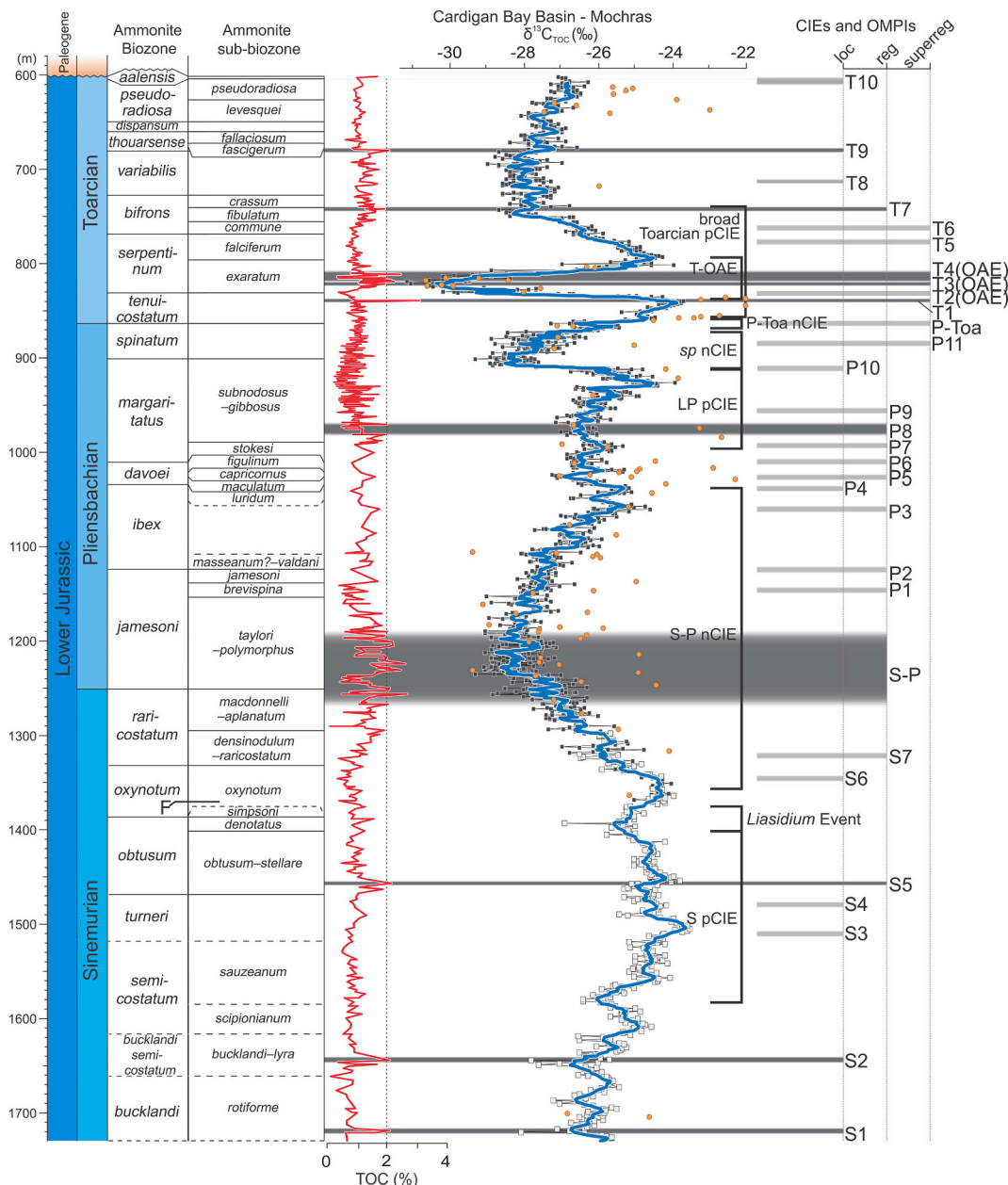
Fig. 4. \delta^{13}\text{C}_{\text{TOC}} , TOC, and projection of OMPs for the Sinemurian–Toarcian at the reference Llanbedr (Mochras Farm) core, Cardigan Bay Basin (modified from Xu et al., 2018; Storm et al., 2020). The dark grey bars refer to OMPs observed at Mochras whereas the light grey bars reflect the approximate position of OMPs against the \delta^{13}\text{C}_{\text{TOC}} curve. Blue line = seven-point moving average. Black squares = samples taken from core slabs; white squares = samples taken from reserve bags (~1.4-m intervals) of broken core. Orange circles = \delta^{13}\text{C}_{\text{wood}} . Depth of the samples from reserve bags refers to midpoint of the sample interval. Ammonite biostratigraphy after (Ivimey-Cook, 1971; Copestake and Johnson, 2013). Loc – Local; reg – regional; superregional; S – Sinemurian; P – Pliensbachian; LP – Late Pliensbachian; sp – spinatum; P-TOA – Pliensbachian–Toarcian; T-OAE – Toarcian oceanic anoxic Event; T – Toarcian; pCIE – positive carbon isotopic excursion; nCIE – negative carbon isotopic excursion; OMPi – organic matter preservation interval; F – fault.
