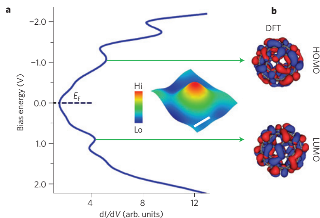
Figure 2 | C_{60} energy levels on n\text{-C}_{30}\text{H}_{62} -coated Au(111). a , Differential conductance ( dI/dV ) spectrum of the C_{60} molecules adsorbed on organic spacer-coated Au(111) in silicone oil medium revealing well-resolved frontier molecular orbitals (feedback loop parameters I = 100 pA, V = 1.2 V). Inset shows a three-dimensional in situ STM image of a single C_{60} molecule over which the dI/dV spectra were recorded (tunnelling set point I = 8 pA, V = 0.4 V, scale bar, 0.6 nm). b , Corresponding DFT-calculated highest occupied molecular orbital (HOMO) and lowest unoccupied molecular orbital (LUMO) of the gas-phase C_{60} molecule.
