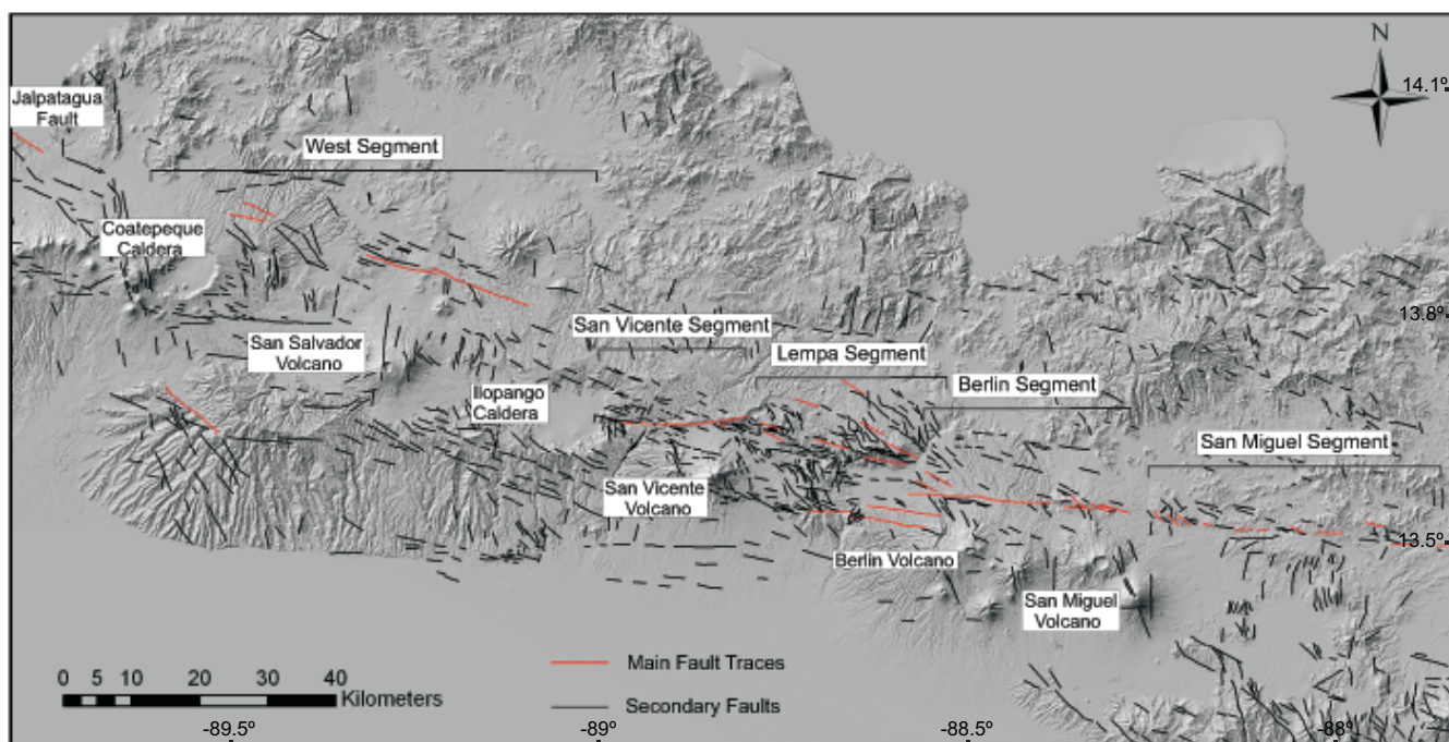
FIGURE 2 | Active fault strands and segments of the El Salvador Fault Zone overlaid onto ten-metre-resolution Digital Terrain Model (DTM) derived from 1:25,000 topographic map.
