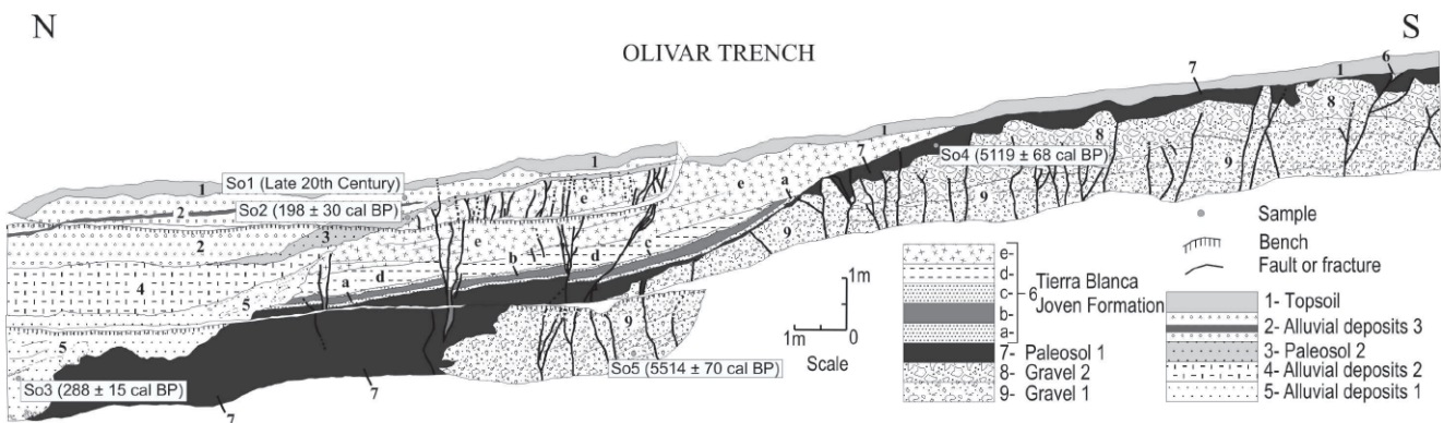
FIGURE 9 | El Olivar trench log (east wall) on the eastern end of the San Vicente segment of the El Salvador Fault Zone. See text for description and Figure 4 for location.
