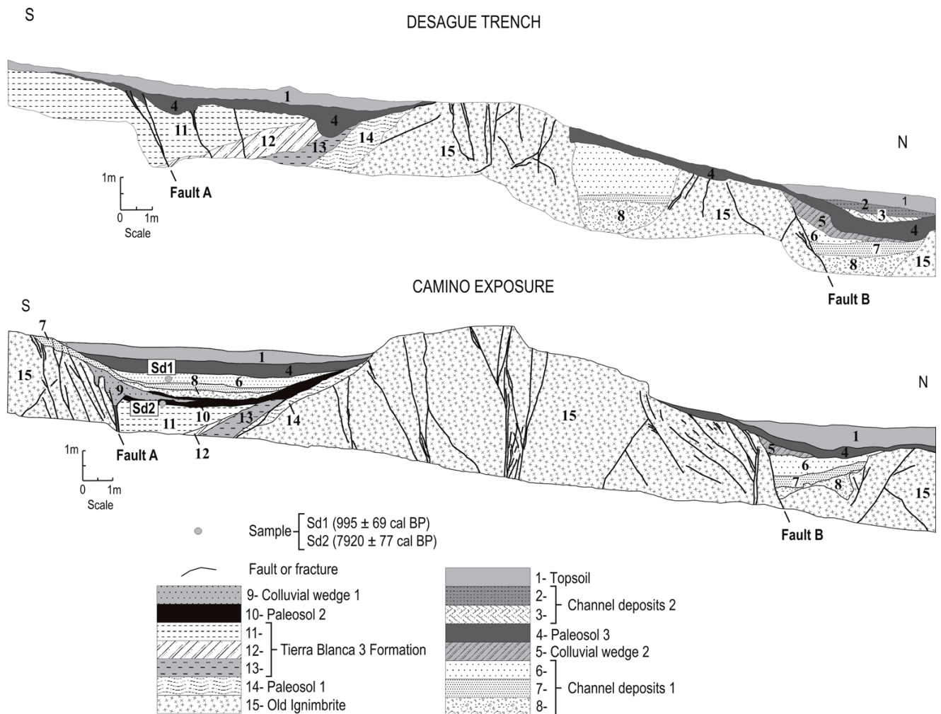
FIGURE 11 | Logs of Desague trench (west wall) and Camino road cut (east wall) on the western end of the San Vicente segment of the El Salvador Fault Zone. See text for description and Figure 4 for location.
