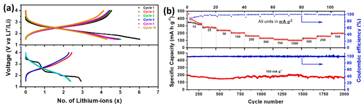
Fig. 5. Electrochemical performance of V_4O_9 against lithium between 1.5 – 4.0 V. (a) charge-discharge plots of V_4O_9 and V_2O_5 nanoparticles; (b) Rate test of V_4O_9 nanoparticles at different current densities and long cycle stability at 100 \text{ mA g}^{-1} .
