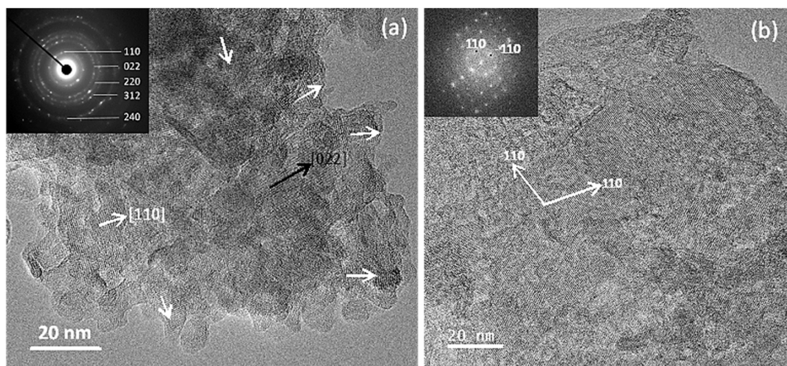
Fig. 3. (a) High resolution micrograph of a nanocrystal agglomerate. Inset shows the corresponding ring electron diffraction pattern indexed on the basis of the Cmc2h structure symmetry of V_4O_9 ; (b) Crystallite oriented close to [001]. FFT in the inset illustrates the almost single crystal nature of the particle.
