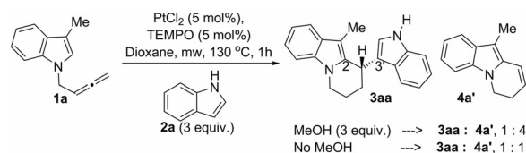
Scheme 8. Experiments in the presence of TEMPO.
