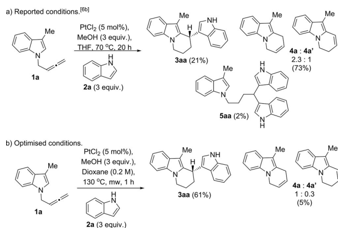
Scheme 2. Platinum-catalysed reaction of 3-methyl- N -(2,3-butadienyl)indole with an external indole: using reported conditions for bisindolylolation of allenes (a) [6b] and optimised conditions (b).
