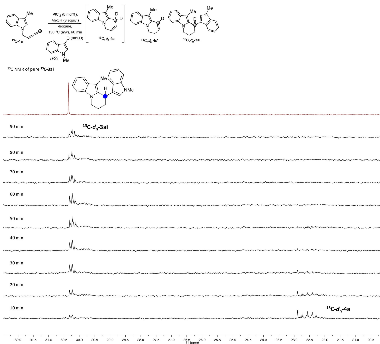
Figure 2. Expansion of the ^{13}\text{C} NMR of the reaction of ^{13}\text{C} - 1a and d-2i over time showing deuterium incorporation in the labelled carbon in 3ai and 4a . See Supporting Information for the signal of labelled carbon in 4a' .
