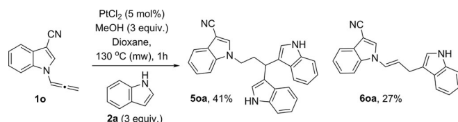
Scheme 3. Reaction of indolylallene 1o with a shorter chain.
