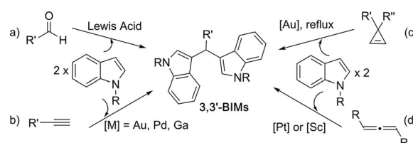
Scheme 1. Different approaches to the synthesis of 3,3'-BIMs.
