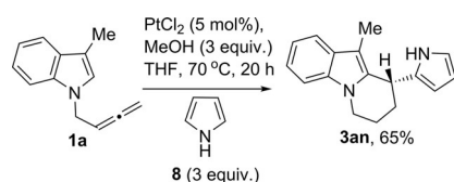
Scheme 5. Further scope with pyrrole.
