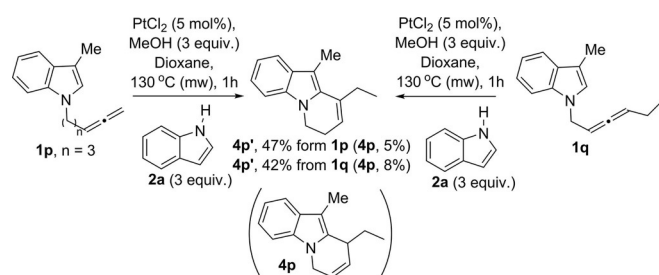
Scheme 4. Reaction of indolylallenes 1p and 1q under optimised conditions.
