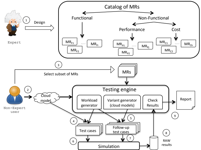
Fig. 1. Architecture of the TEA-Cloud framework
