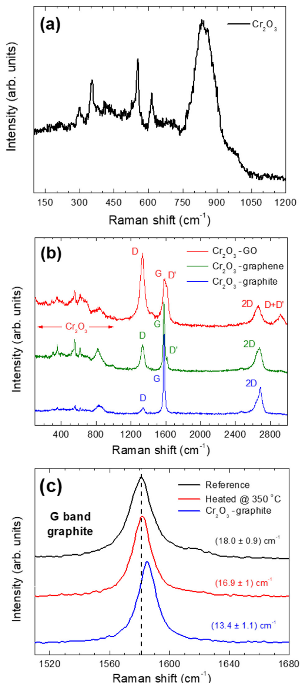
Fig. 2. Raman spectra of \text{Cr}_2\text{O}_3 nanoparticles obtained at 350 °C (a) and their composites with graphite, graphene and GO (b). (c) Detail of the G band observed in Raman spectra of pristine graphite, graphite annealed at 350 °C and a \text{Cr}_2\text{O}_3 -graphite composite. FWHM of each band is indicated above the corresponding spectrum.
