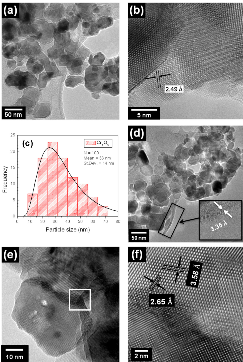
Fig. 3. (a) Low magnification TEM image of the investigated \text{Cr}_2\text{O}_3 nanoparticles. (b) HRTEM micrograph showing the crystalline nature of the obtained oxide. (c) \text{Cr}_2\text{O}_3 particle size distribution histogram and lognormal fitting. (d) Low magnification TEM image of the \text{Cr}_2\text{O}_3 -graphene composite showing the oxide nanoparticles distributed on the carbon layers. Stacked carbon layers can be observed in the inset. (e) HRTEM micrograph of a chromia nanoparticle in the \text{Cr}_2\text{O}_3 -graphite sample. (f) HRTEM image of the area marked in Fig. 3 (e).
