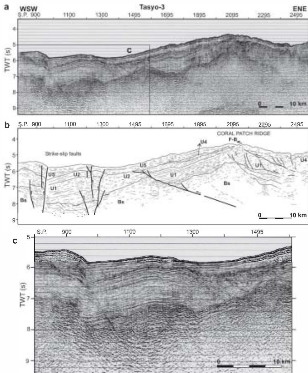
Fig. 9. MCS line Tasyo-3 (a) and line drawing (b) at the Coral Patch Ridge. Discussion in the text. Black box on the MCS line outlines a detailed section (c). See Fig. 1 for location and Fig. 4 for seismic units explanation.
