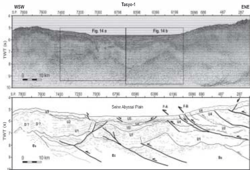
Fig. 13. Western segment of MCS line Tasyo-1 and line drawing. Details of interpretation in text. D: Diapirs. The black boxes on the MCS line outline detailed segments depicted in Fig. 14. See Fig. 1 for location and Fig. 4 for seismic units explanation.
