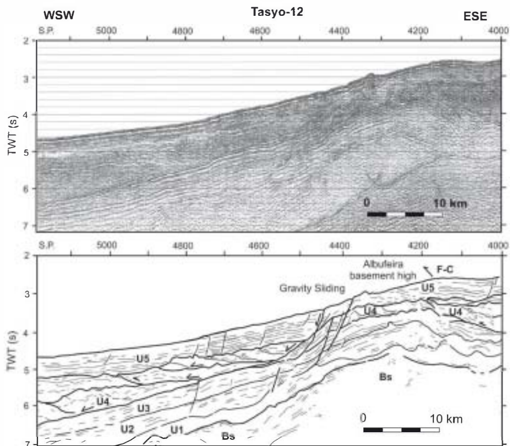
Fig. 7. Segment of MCS line Tasyo-12 and line drawing. Note the slope failure produce by gravity-driven advance of the allochthonous sheets at the base of the Albufeira High. See Fig. 1 for location and Fig. 4 for seismic units explanation.
