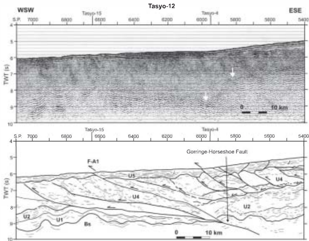
Fig. 8. Segment of MCS line Tasyo-12. Note the Gorringe–Horseshoe fault, which marks a change in the basement dip. Arrows denote the offset produced by the fault. See Fig. 1 for location and Fig. 4 for seismic units explanation.
