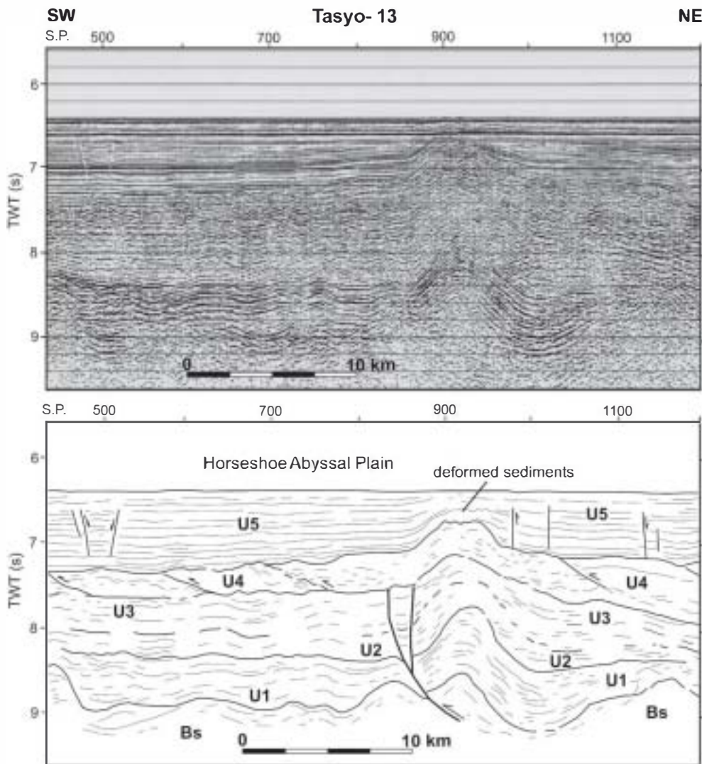
Fig. 12. MCS line Tasyo-13 and line drawing showing a blind basement thrust at the Horseshoe Abyssal Plain. Details of interpretation in text. See Fig. 1 for location and Fig. 4 for seismic units explanation.
