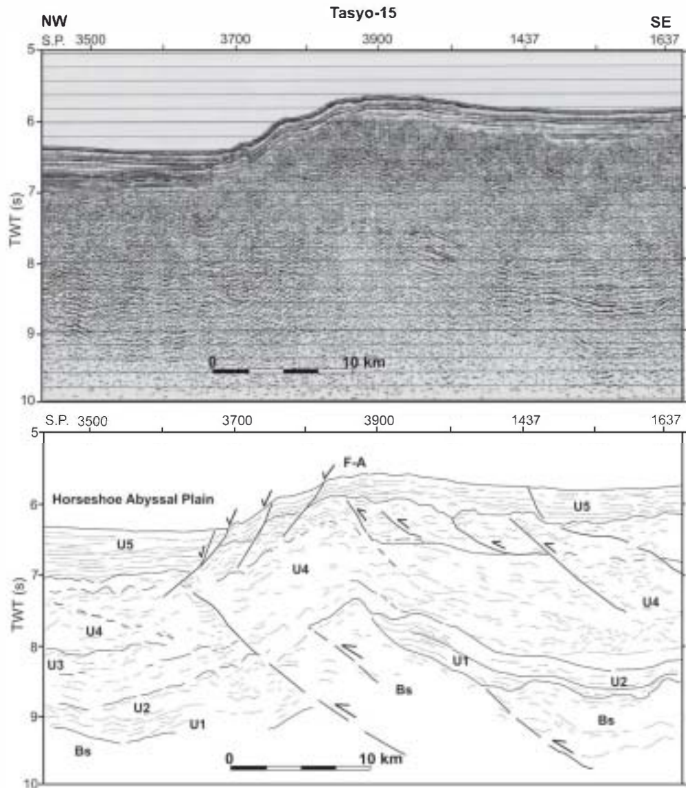
Fig. 11. MCS line Tasyo-15 and line drawing showing the thrust fault that marks the eastern boundary of the Horseshoe Abyssal Plain. Associated recent slides are observed. This thrust fault has also been cut southwards by line Tasyo 12 (Fig. 10, S.P. 7900). Details of interpretation in text. See Fig. 1 for location and Fig. 4 for seismic units explanation.
