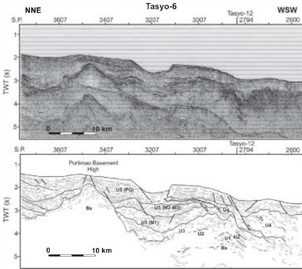
Fig. 6. Detail of the MCS line Tasyo-6 and line drawing in the Portimao basement high area, showing the external front of the AUGC. See Fig. 1 for location and Fig. 4 for seismic units explanation.
