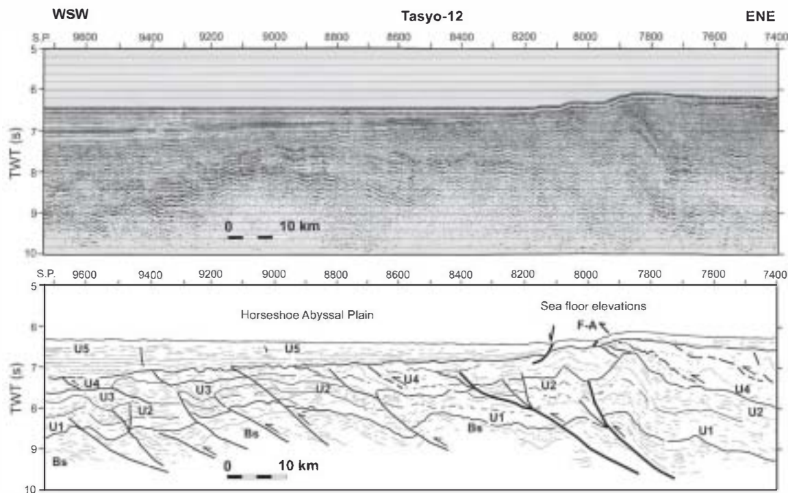
Fig. 10. Western segment of MCS line Tasyo-12 and line drawing showing the thrust belt of the Horseshoe Abyssal Plain. Details of interpretation in text. See Fig. 1 for location and Fig. 4 for seismic units explanation.
