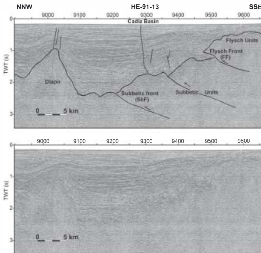
Fig. 5. Interpreted MCS line HE-91-13 and seismic profile across the Flysch and Subbetic units. Discussion in the text. See Fig. 1 for location.
