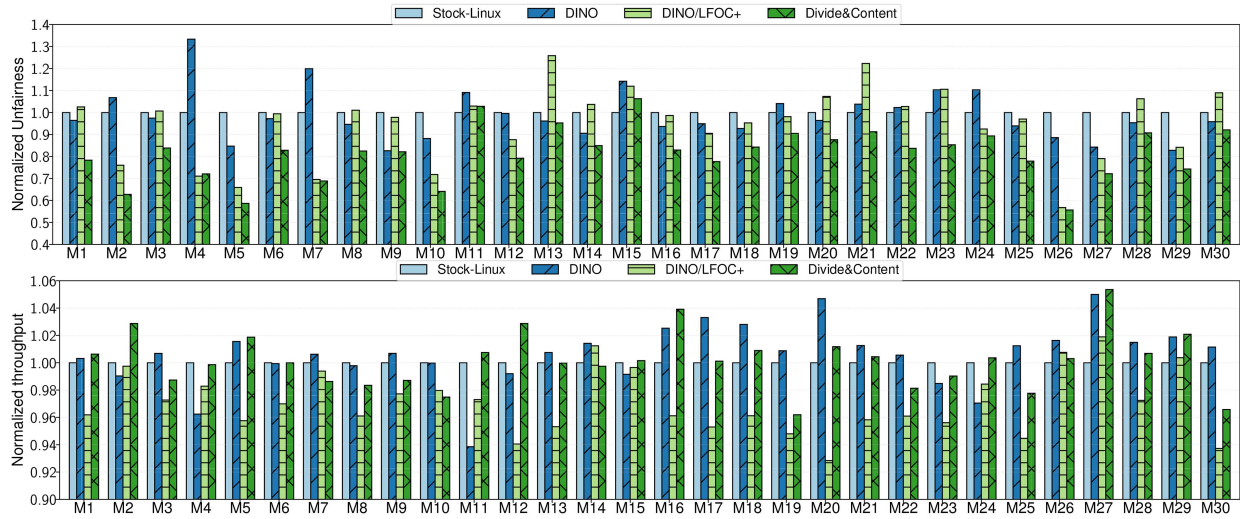
Fig. 10. Normalized unfairness and STP values obtained by the various strategies.
