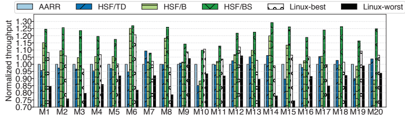
Fig. 3. Normalized throughput delivered by the various scheduling algorithms
