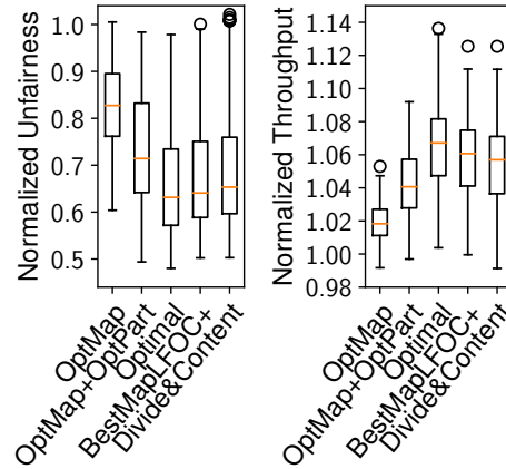
Figure 3.5: Unfairness and throughput distribution for the normalized simulation results, with 240 workloads across four theoretical solutions.
