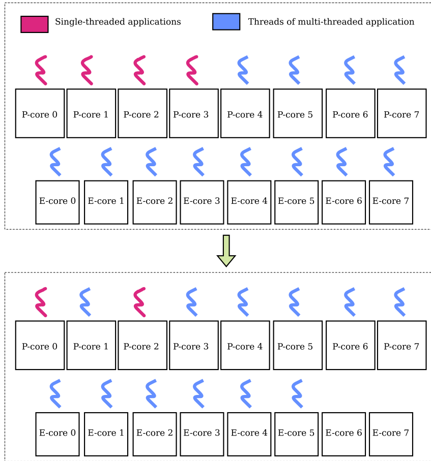
Figure 3.23: Scenario illustrating HSP and Flexible AID in action on a 16-core system (half P-cores and half E-cores).
