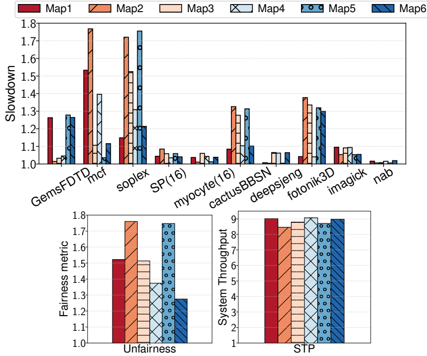
Figure 3.2: Per-application slowdown (top) and unfairness and throughput (bottom), for 6 different thread-to-LLC mappings of a 10-application workload under the LFOC+ LLC-partitioning policy. The numbers in parentheses by SP and myocyte (parallel) indicate their thread count.
