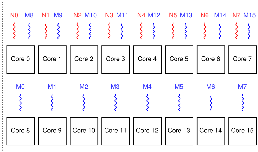
Figure 3.11: Oversubscription scenario: 8 threads (N0-N7) belong to program N, and 16 threads (M0-M15) to program M.
