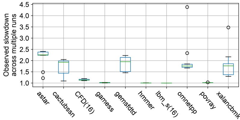
Figure 1.2: Variability of the average observed slowdown across 10 runs of a multi-application workload. Two benchmarks run with multiple threads, their count is listed in parentheses along with the names. The default Linux scheduler was used.
