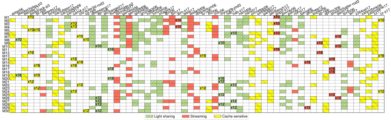
Fig. 9. Each table row M_i depicts the composition of the i -th workload used in our experiments. For each benchmark, the dominant application class observed during the execution is displayed in the associated column. When a program is not included in a workload a blank cell is used in the corresponding row. The “xN” mark indicates that the associated benchmark runs with N threads. A suffix has been added to each benchmark’s name to indicate the corresponding suite (e.g., “17” denotes SPEC CPU2017, “p3” is for PARSEC3 and “-npb” for NAS Parallel Benchmarks).
