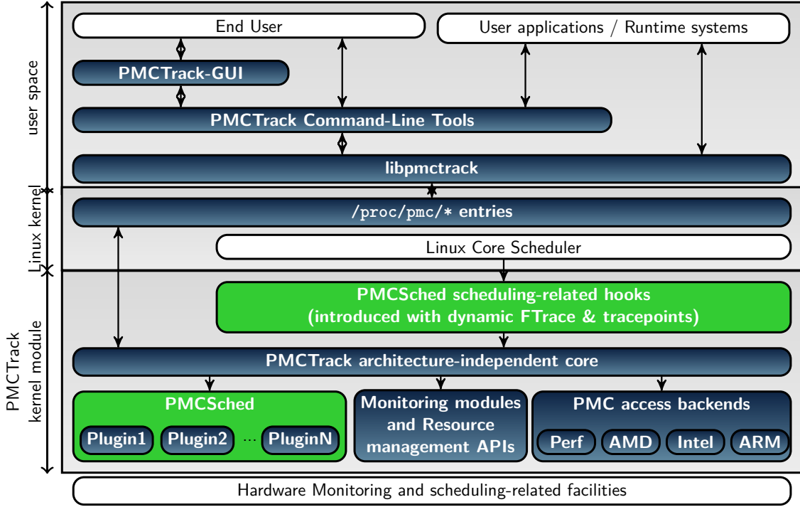
Figure 3.1: Addition of PMCSched within the larger PMCTrack system.
