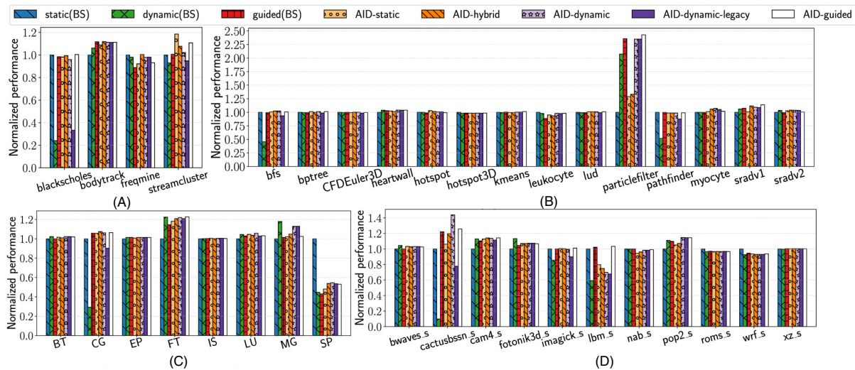
FIGURE 11 Performance of the various OpenMP applications obtained for different loop-scheduling strategies with the BS mapping normalized to static (BS). (A) PARSEC. (B) Rodinia. (C) NAS parallel benchmarks. (D) SPEC CPU2017.
