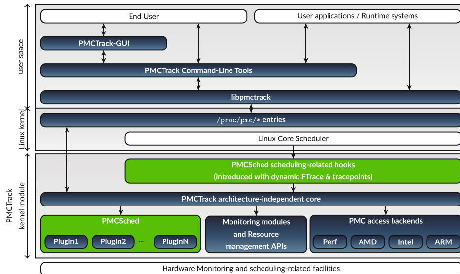
FIGURE 1 PMCSched components (in green) inside PMCTrack's architecture.
