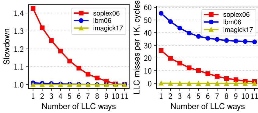
Figure 2.9: Slowdown (left side) and LLCMPKC (right side) for three different applications and varying numbers of cache ways allocated to them. Each application belongs to one of the classes distinguished by LFOC+: cache-sensitive ( soplex , in red) streaming ( lbm , in blue), and light-sharing ( imagick , in green).
