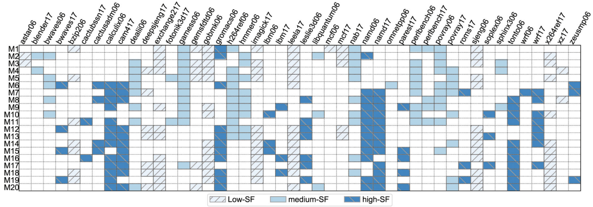
FIGURE 7 Workloads used for our experiments. Each row M_i depicts the composition of the i th workload. A blank cell indicates that the associated program is not included in the workload. Applications whose average SF is lower than 1.7 are considered low-SF programs in our platform, and those with an SF value greater than 2.05 are classified as high-SF. The remaining ones are labeled as medium-SF.
