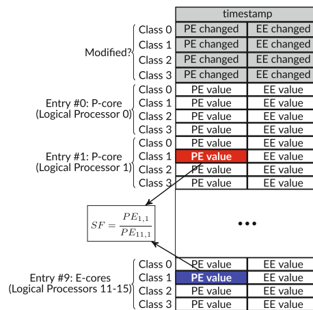
FIGURE 3 Structure of the Thread Director table on our Alder Lake experimental platform.
