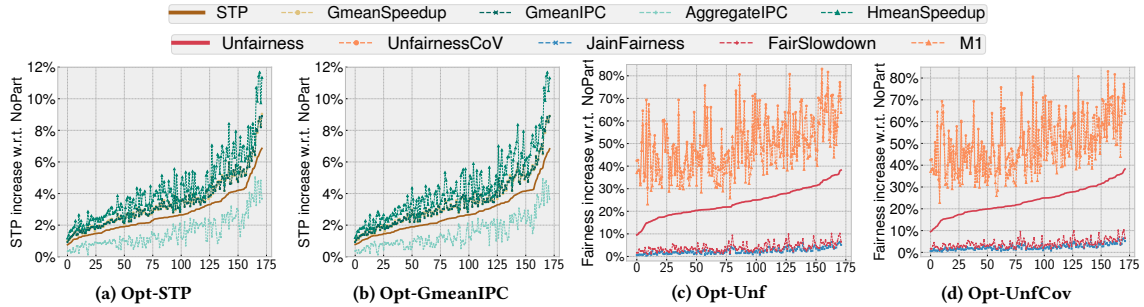
Figure 2: Correlation between throughput and fairness metrics across workloads and optimization objectives, sorted by STP gains –charts (a) and (b)– and Unfairness reductions –charts (c) and (d).
