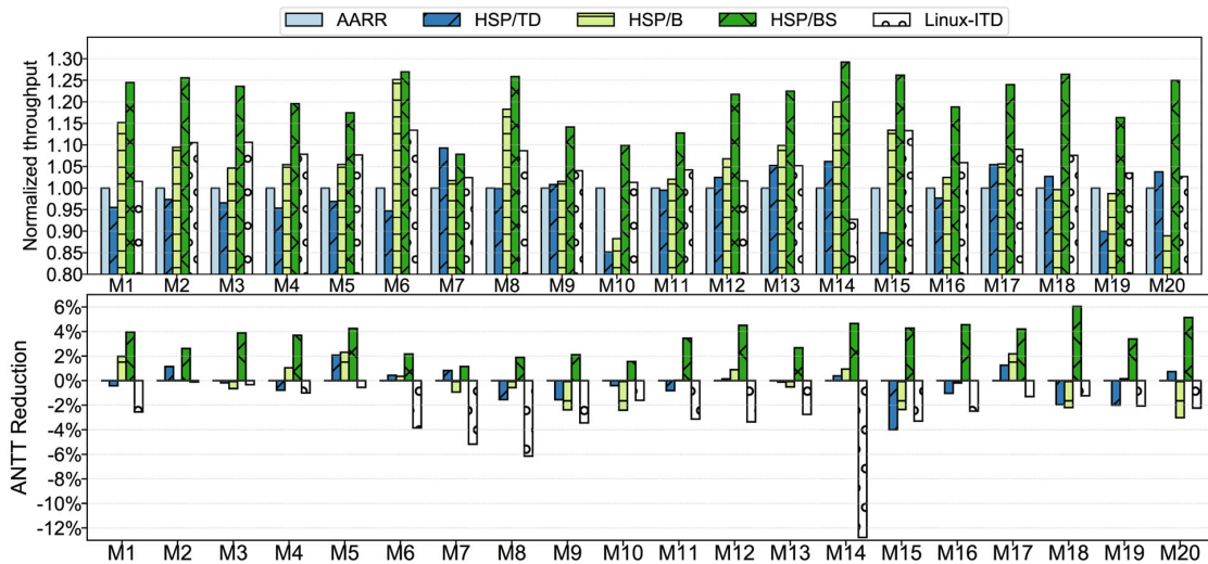
FIGURE 8 Normalized throughput and ANTT reduction associated with the various scheduling algorithms.
