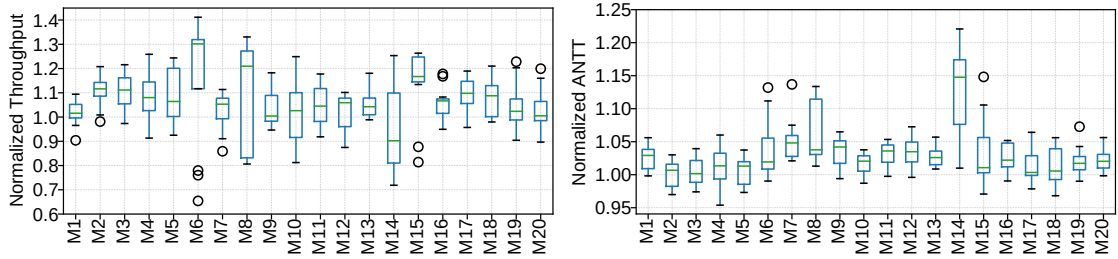
Figure 3.21: Distribution of normalized throughput (higher is better, left side) and ANTT values (lower is better, right side) under multiple runs of Linux-ITD.
