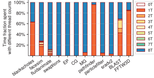
Figure 2: Time fraction spent with different runnable thread counts in various applications.
