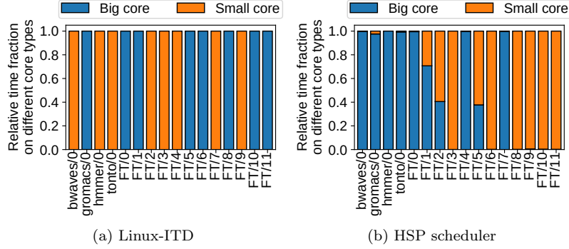
Figure 3.25: Relative time each W2 threads spends on core types under different OS schedulers. The x-axis labels show the program name and TID, separated by a slash.
