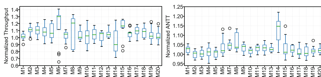
FIGURE 9 Distribution of normalized throughput (higher is better) and ANTT values (lower is better) under multiple runs of Linux-ITD.
