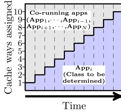
Figure 2.10: Distribution of the LLC space over time during the LFOC+’s sampling mode for App_i . Figure reproduced from LFOC+’s literature [136].
