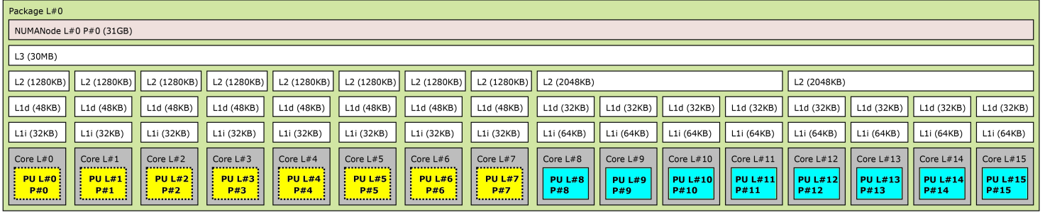
Figure 2.3: Topology of the AlderLake-16 platform.
