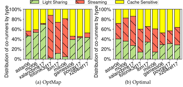
Fig. 6. Distribution of co-runners (by type) assigned to the same core group for 9 selected programs—3 sensitive, 3 streaming and 3 light sharing (in the order used in the x axis)—, under OptMap and Optimal.
