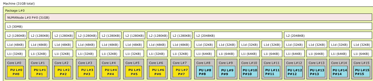
FIGURE 2 The system employed in our experiments. The eight E-cores (right side in blue color) are grouped into two 4-core clusters, sharing a 2 MB L2 cache. P-cores (left side in yellow color) have a private 1.25 MB L2 cache. All E-cores and P-cores share a 30 MB L3 (LLC).
