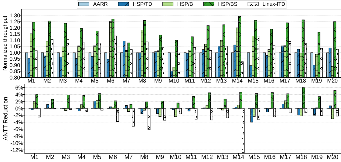
Figure 3.19: Normalized throughput and ANTT reduction associated with the various scheduling algorithms.
