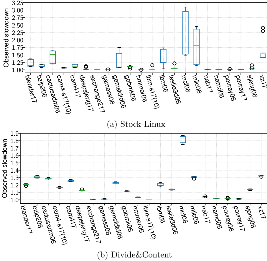
Figure 3.7: Distribution of the per-application slowdown for one of the tested workloads under Stock-Linux (a) and Divide&Content (b).
