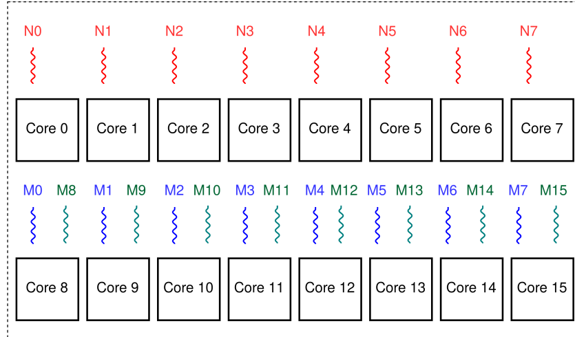
Figure 3.12: EM scenario: 8 threads (N0-N7) belong to the Non-Malleable (N) program, and 8 threads (M0-M7) to the Malleable (M) program. Eight additional worker threads are also created (M8-M15) but they are initially inactive (in green).
