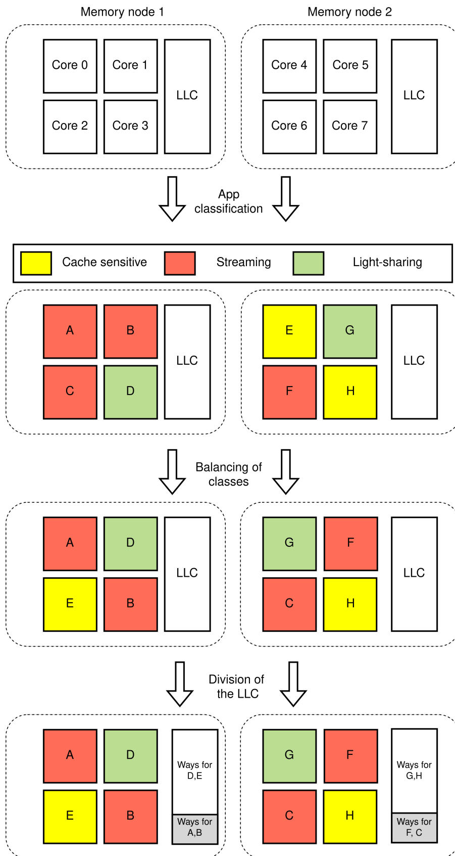
Figure 3.6: High-level overview of the contention balancing algorithm of Divide&amp;Content.
