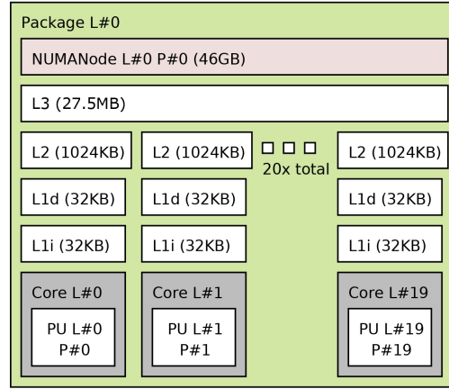
Figure 1.1: Cache hierarchy of the Intel Xeon Gold 6138 “Skylake” processor.
