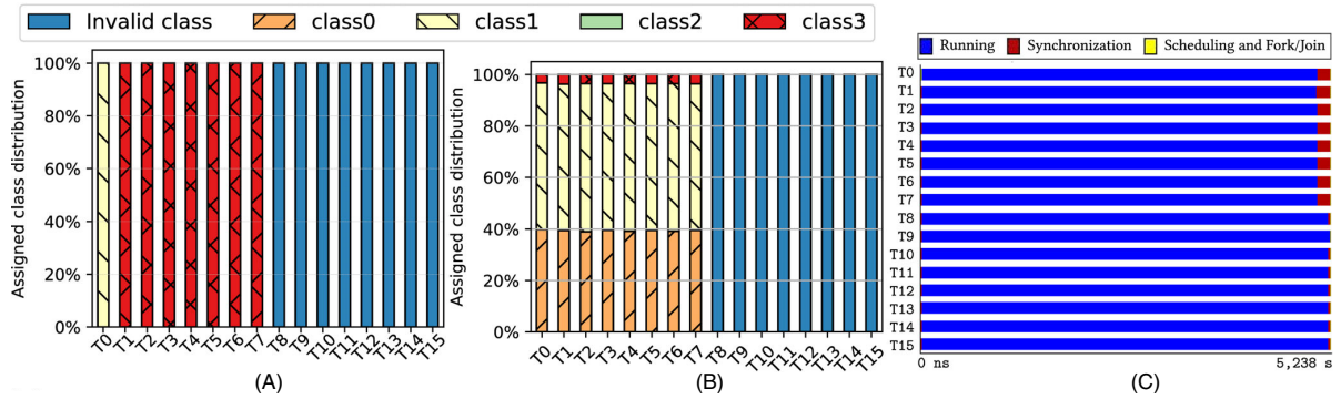
FIGURE 5 Demonstration of the effectiveness of the spin-loop detection feature in Thread Director with (A) the barrier microbenchmark and (B) the EP program. (C) Depicts the load imbalance situation under EP that leads T0–T7 threads to busy wait for a while. (A) Class distribution for threads in barrier. (B) Class distribution for threads in EP. (C) Execution trace of EP.
