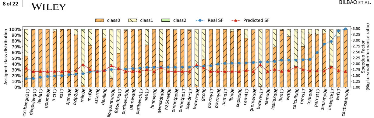
FIGURE 4 Proportion of assigned classes on big cores versus actual and TD-predicted speedup factor.
