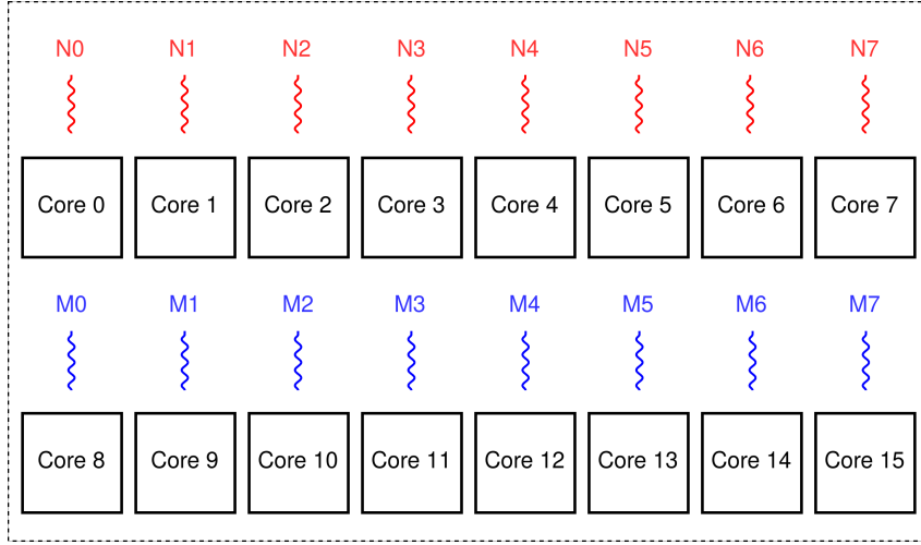
Figure 3.10: Stock-Linux scenario: 8 threads (N0-N7) belong to non-malleable program N, and 8 threads (M0-M7) to malleable program M.
