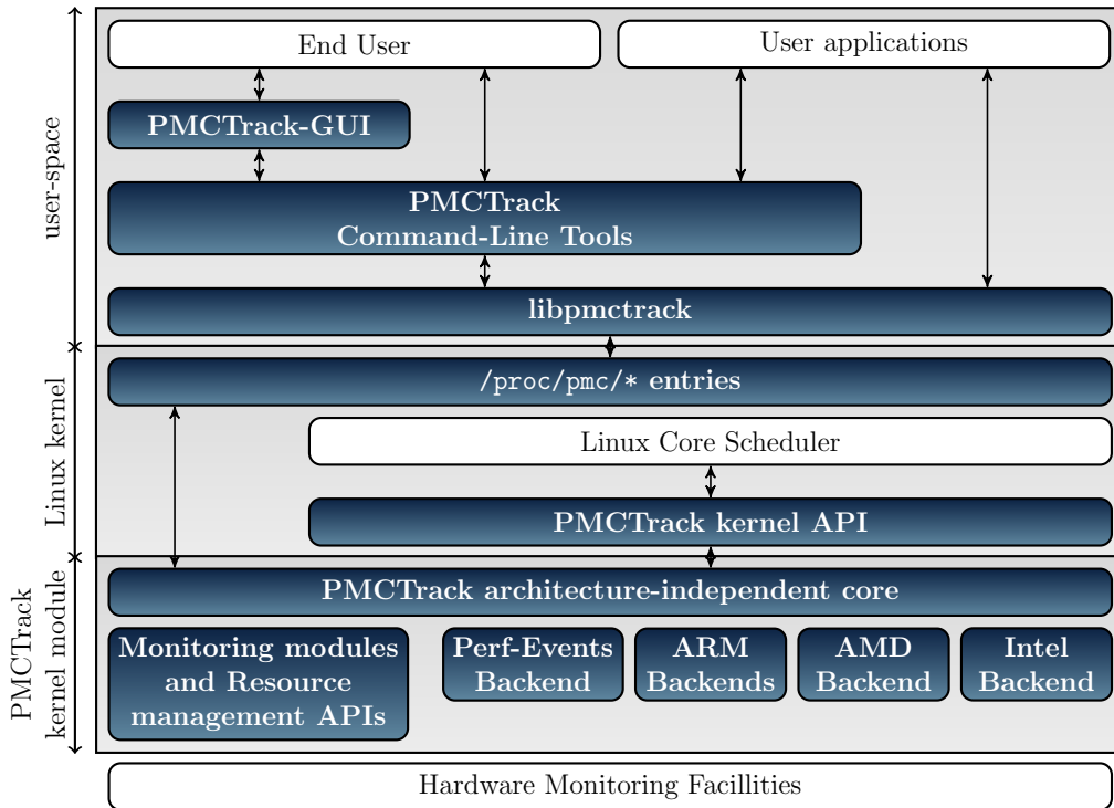
Figure 2.5: Architecture and main components of the PMCTrack tool (before the adoption of the PMCSched framework).
