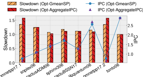
Figure 3: Slowdown and IPC of various co-running programs delivered by Opt-GmeanSP and Opt-AggregateIPC.
