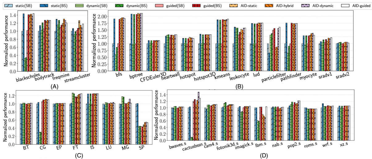
FIGURE 10 Normalized performance of the various OpenMP applications obtained for different loop-scheduling strategies. (A) PARSEC. (B) Rodinia. (C) NAS parallel benchmarks. (D) SPEC CPU2017.
