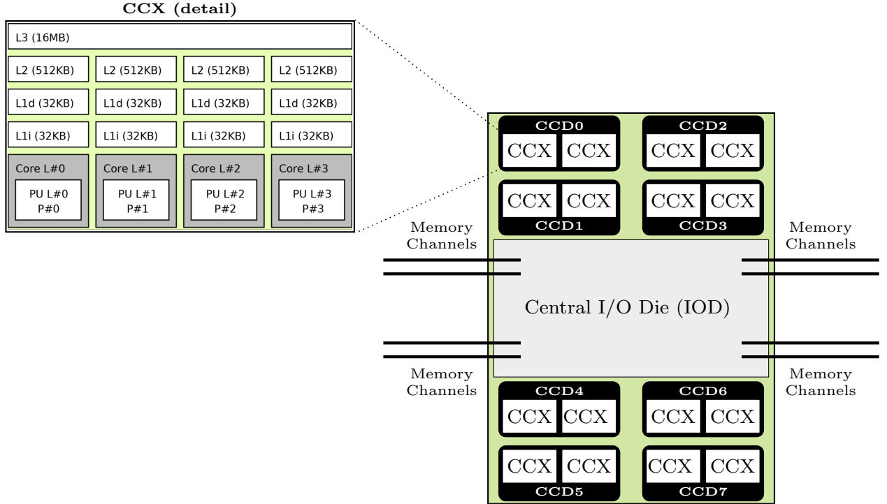
Figure 2.4: Topology of one socket of the Zen2-128 platform.
