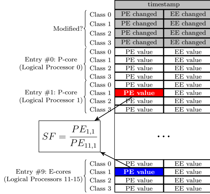
Figure 3.15: Structure of the Thread Director table in our Alder Lake experimental platform.
