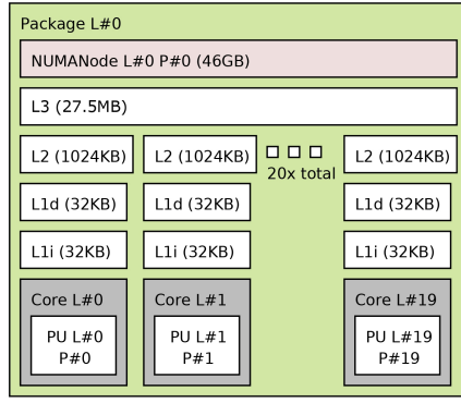
Figure 2.1: Topology of one of the two NUMA nodes of Skylake-40.
