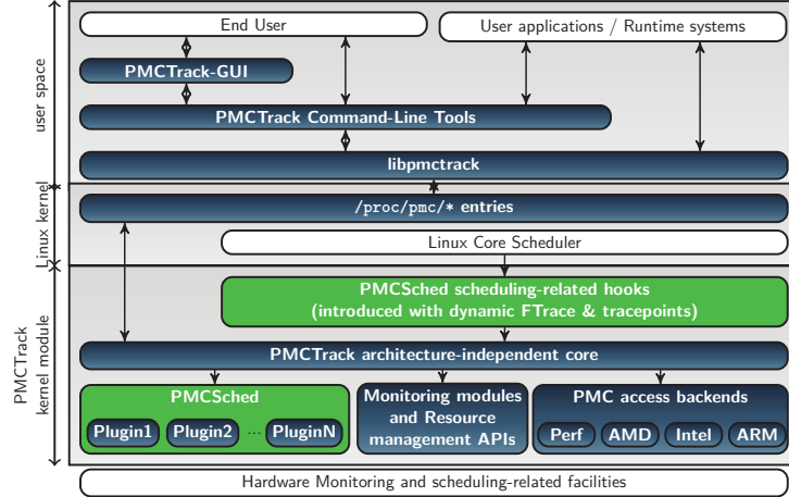
Fig. 1. PMCSched components (in green) inside PMCTrack's architecture.
