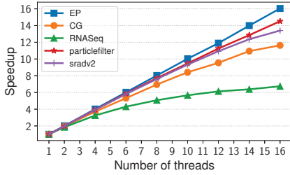
Figure 3: Scalability of several OpenMP programs in our experimental platform.
