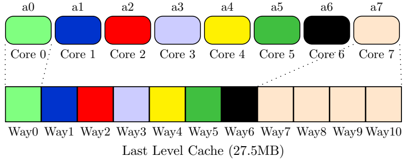
Figure 2.6: Example of strict cache-partitioning, with 8 applications (a0-a7) each running on a separate core and LLC partition.
