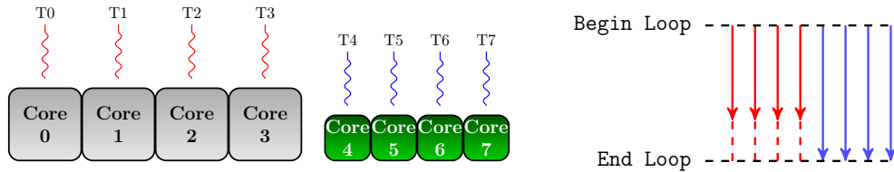
Figure 3.17: Typical imbalance scenario of a regular loop-based parallel program running on an AMP system.
