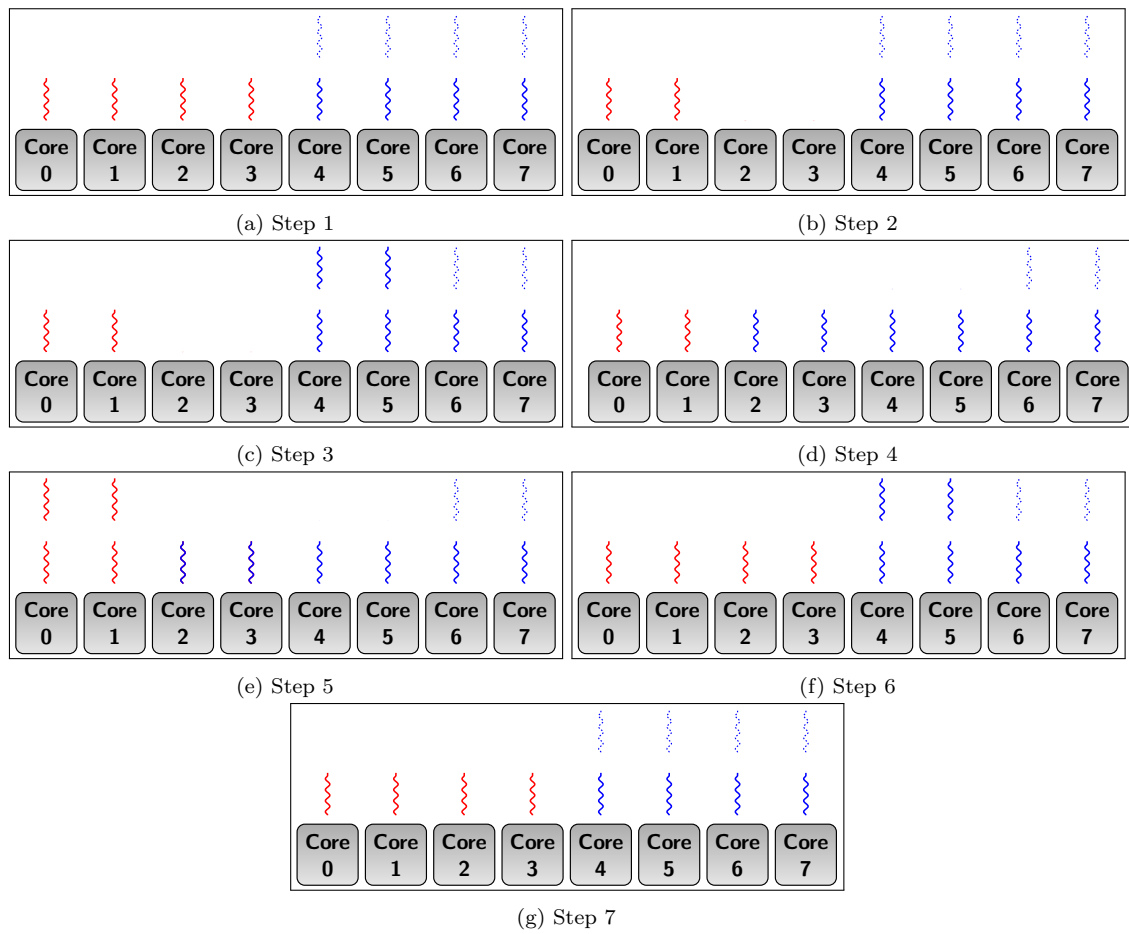
Figure 3.9: Elasticity Manager in action with two applications running on an 8-core system.
