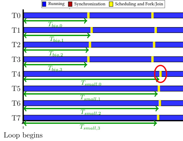
Figure 3.18: Example of AID sampling period, with four worker threads running on big cores and four threads assigned to small cores.
