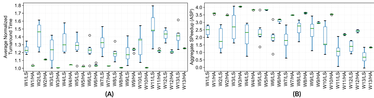
FIGURE 13 Distribution of (A) average normalized turnaround time (ANTT) and (B) throughput (ASP metric) for the various workloads under Linux-ITD with standard OpenMP (LS) and HSP with AID loop-scheduling methods (HA).
