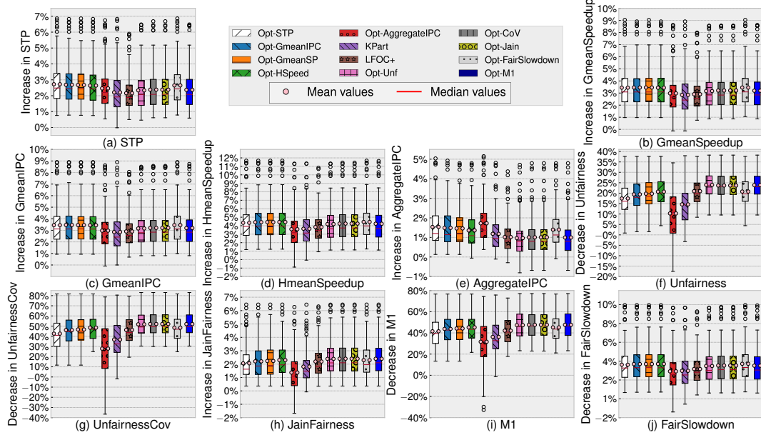
Figure 1: Distribution of improvements for the various metrics with respect to NoPart for the different schemes.
