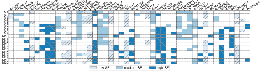
Fig. 2. Workloads used for our experiments. Each row M_i depicts the composition of the i -th workload. A blank cell indicates that the associated program is not included in the workload. Applications whose average SF is lower than 1.7 are considered low-SF programs in our platform, and those with an SF value greater than 2.05 are classified as high-SF. The remaining ones are labeled as medium-SF.
