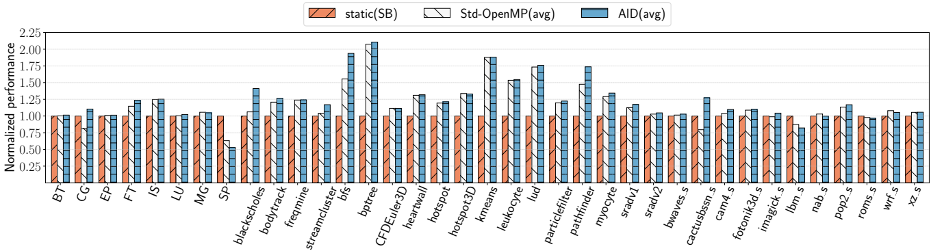
Figure 3.22: Average normalized performance across all standard OpenMP methods (std-OpenMP) and across all AID strategies for all the OpenMP programs explored.
