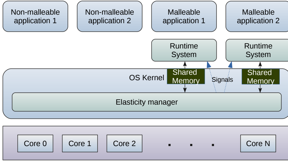
Figure 3.8: Diagram of the elasticity manager, including the shared memory region for communication between the runtime and the elasticity manager.
