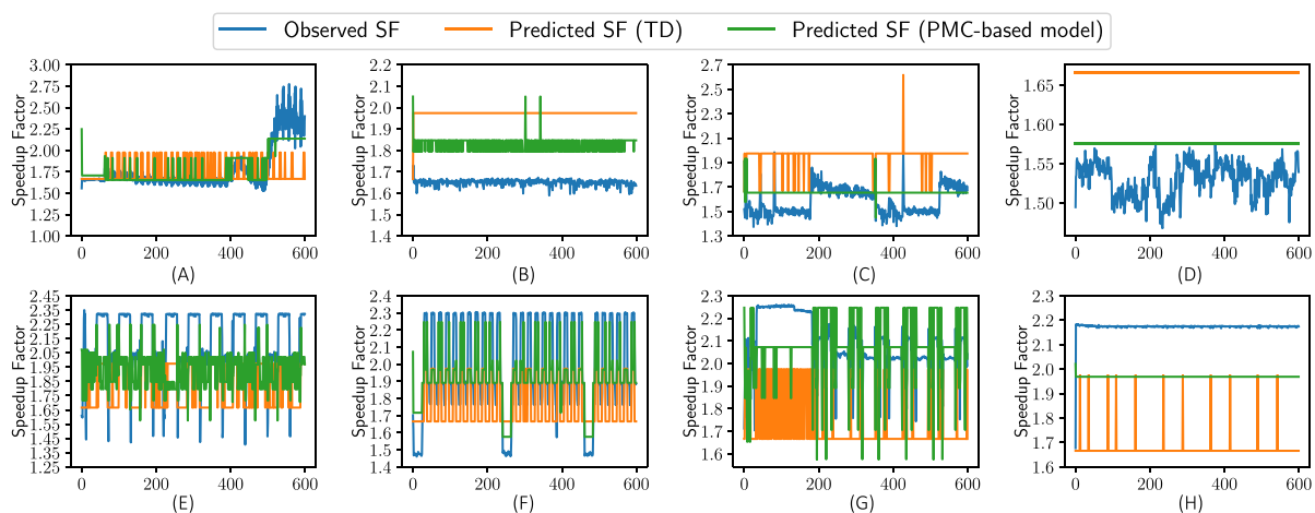
FIGURE 6 Comparison between real speedup factor (SF) and that predicted by TD and a PMC-based model 4 on big cores. The figure plots the predictions observed over time for a total of 30B instructions (SF values sampled every 50M retired instructions). Actual SF values are obtained with the IPC ratio of each 50M-instruction window gathered on both core types, as explained in detail in our earlier work. 4 (A) fotonik3d17. (B) imagick17. (C) milc06. (D) sjeng06. (E) calculix06. (F) nab17. (G) cam417. (H) lbm17.
