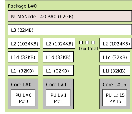
Figure 2.2: Topology of the CascadeLake-16 platform.
