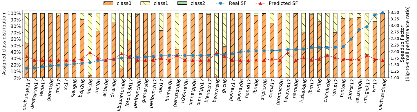
Figure 3.16: Proportion of assigned classes on big cores compared to actual and predicted speedup factor (SF) by Intel Thread Director.
