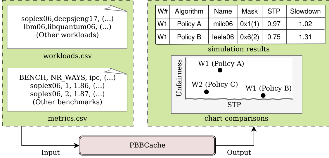
Figure 2.8: Input files for PBBCache (left side, workloads.csv and metrics.csv ) and generated output (right side, simulation results and graphics).
