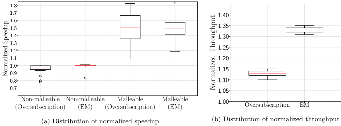
Figure 3.14: Distribution of the relative speedup (a) and normalized throughput (b) between oversubscription and the elasticity manager (normalized to Stock-Linux).
