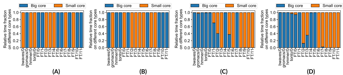
FIGURE 14 Relative time fraction that each thread on W2 spends on the different core types throughout its execution under the different OS schedulers. The labels found in the x-axis indicate the program's name and the TID, both separated by a slash. (A) Linux-ITD (Run1). (B) Linux-ITD (Run2). (C) HSP scheduler (Run1). (D) HSP scheduler (Run2).
