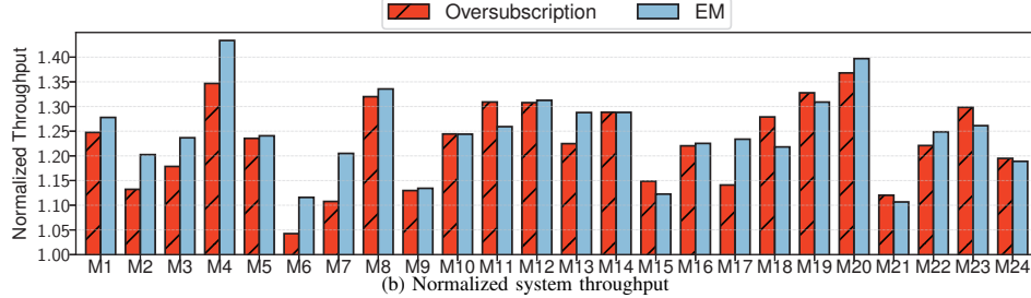
Figure 4: (a) Relative speedup for each application in the workload under Oversubscription and EM vs. Stock-Linux, and (b) normalized throughput for the various program mixes.
