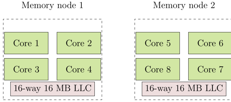
Figure 3.3: Platform A with 8 cores, organized into two four-core memory nodes.
