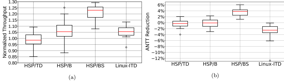
Figure 3.20: Distribution of normalized throughput (a) and ANTT reduction (b) associated with the various scheduling algorithms.
