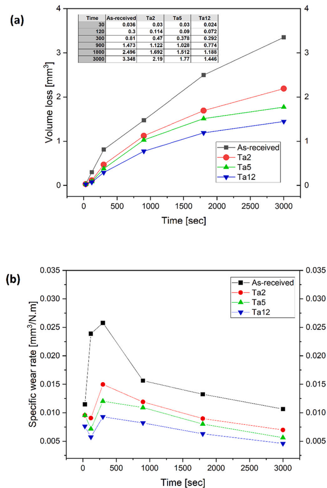
Fig. 6. The influence of sliding time and IEAP pass numbers on the wear behavior of tantalum: (a) volume loss; (b) specific wear rate. The relative error is <13%.
