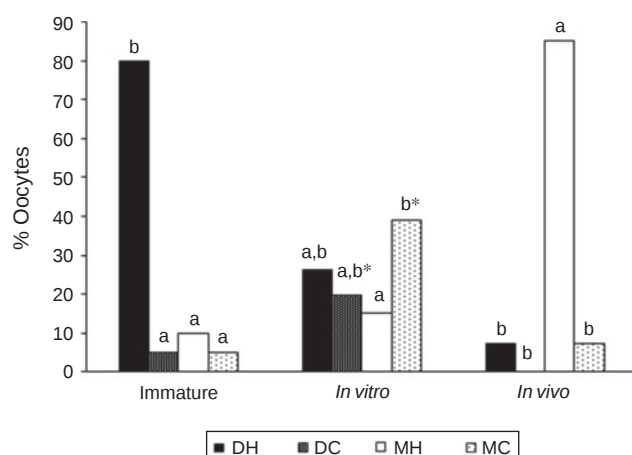
Fig. 4. Percentage of germinal vesicle (immature), IVM and in vivo -matured oocytes exhibiting the different mitochondrial distribution patterns. Within each group, columns with different letters differ significantly. Data with * differs ( P = 0.1 ). DH, diffused homogeneous; DC, diffused clustered; MH, migrated homogeneous; MC, migrated clustered.
