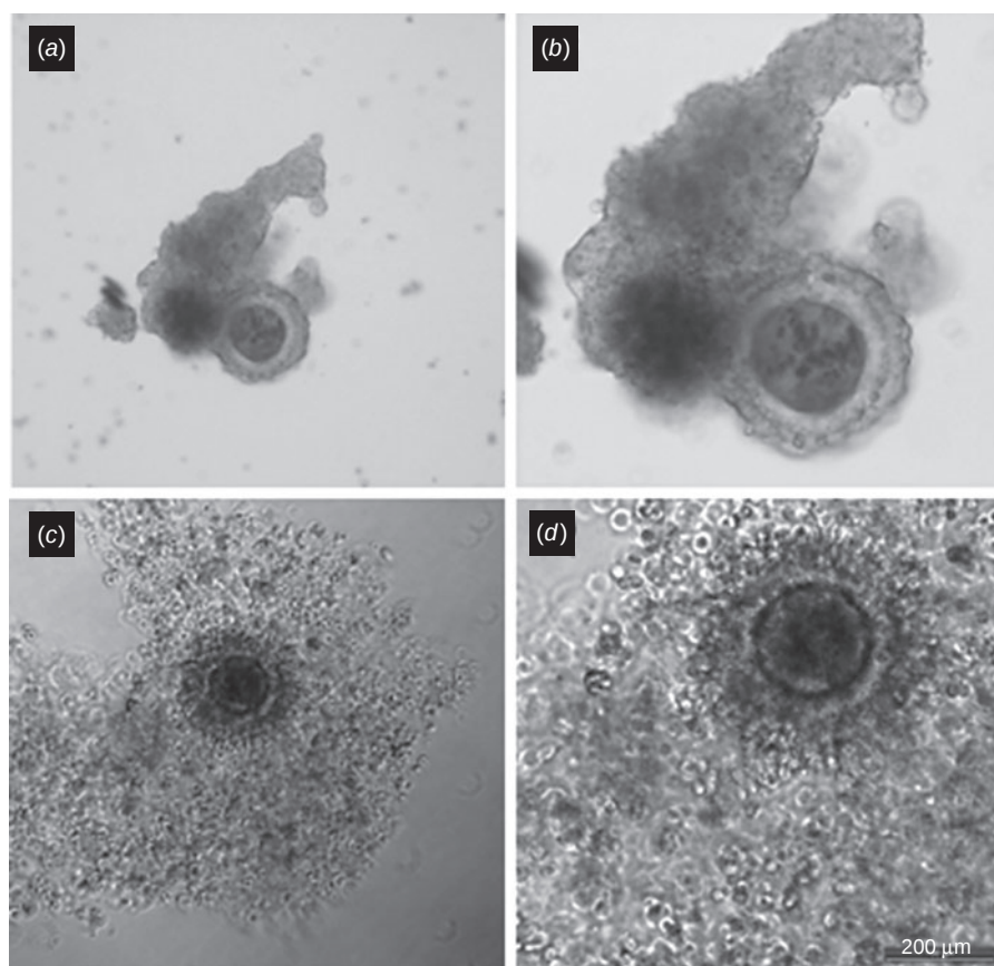
Fig. 6. Cumulus–oocyte complexes after (a, b) IVM or (c, d) in vivo maturation. Scale bar = 200 \mu m.
