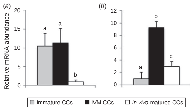
Fig. 1. Relative mRNA abundance of (a) gap junction protein, alpha 1, 43 kDa ( Gja1 ) and (b) prostaglandin-endoperoxide synthase 2 ( Ptgs2 ) in cumulus cells (CCs) of germinal vesicle (immature), IVM and in vivo -matured oocytes. Data are the mean \pm s.e.m. Columns with different letters differ significantly ( P < 0.05 ).
