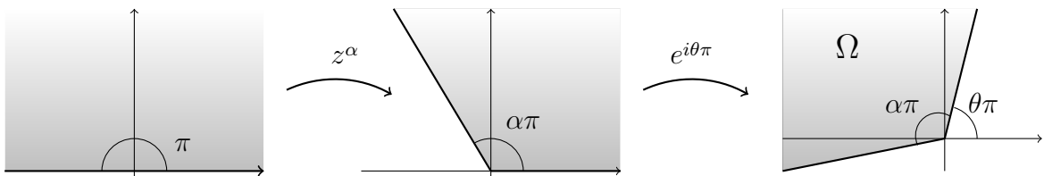
FIGURE 2. Monotone cone with aperture \alpha\pi .
