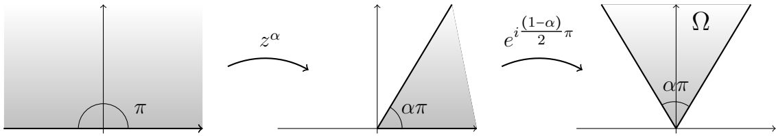
FIGURE 1. Symmetric cone with aperture \alpha\pi .
