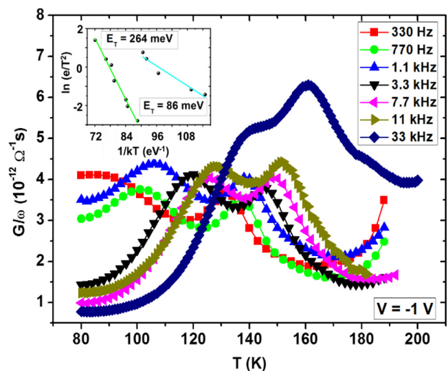
FIG. 3. G/\omega - T curves and the Arrhenius plot corresponding to 10^{14} \text{ cm}^{-2} implantation dose. The bias voltage value is -1 \text{ V} .
