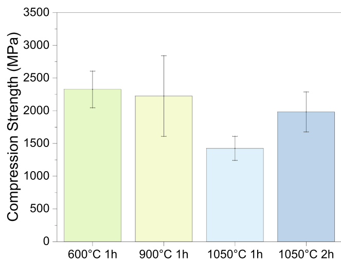
Fig. 9. Compression strength for 10 mol % YSZ micropillars annealed for 1 h at 600 °C, 900 °C, and 1050 °C, and for 2 h at 1050 °C.
