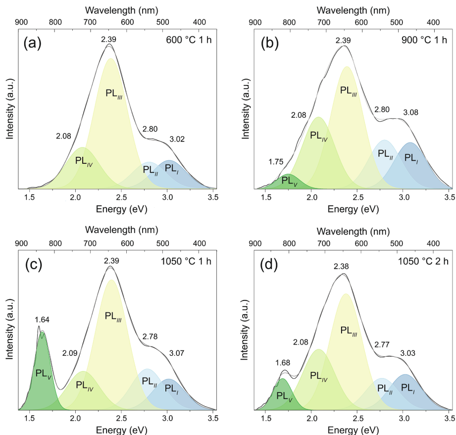
Fig. 6. Deconvoluted μ-PL emission spectra of 10 mol% YSZ octet-truss lattices annealed for 1 h at (a) 600 °C, (b) 900 °C (c) 1050 °C, and for 2 h at (d) 1050 °C.
