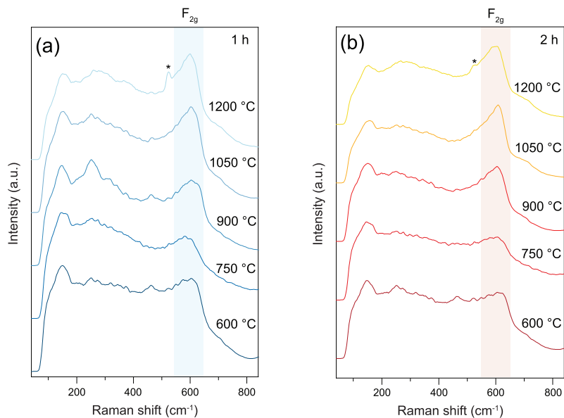
Fig. 5. Raman spectra of 3D structures annealed at 600 °C, 750 °C, 900 °C, 1050 °C, and 1200 °C for (a) one hour and (b) two hours. The F 2g mode region is labeled. A substrate peak (Si) is detected in some cases, noted with an asterisk (*).
