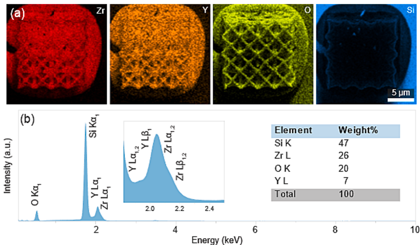
Fig. 4. (a) SEM-EDX images showing the distribution of Zr, Y, O, and Si throughout the octet-truss lattice printed on a Si substrate annealed at 1050\text{ }^{\circ}\text{C} for 2 h, and (b) corresponding EDX spectrum.
