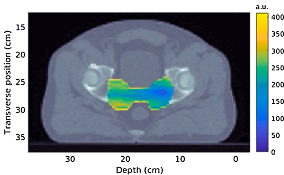
Fig. 2. Example error mask \varepsilon(i, j) corresponding to each pencil beam in the dictionary (eq. 4), overlaid on a CT axial image, for a set of 4 signals, which in this example case are taken from the dictionary \{D_1(t; 13.5; 27), D_2(t; 13.5; 27), D_3(t; 13.5; 27), D_4(t; 13.5; 27)\} , captured at detectors placed on positions referred to in Fig. 3. Within this mask, dark blue represents lowest values of error, i.e. positions where it is most likely to find the Bragg peak, and yellow represents highest values of error, that is positions situated further away from the Bragg peak, according to the measured signals. (For interpretation of the references to colour in this figure legend, the reader is referred to the web version of this article).
