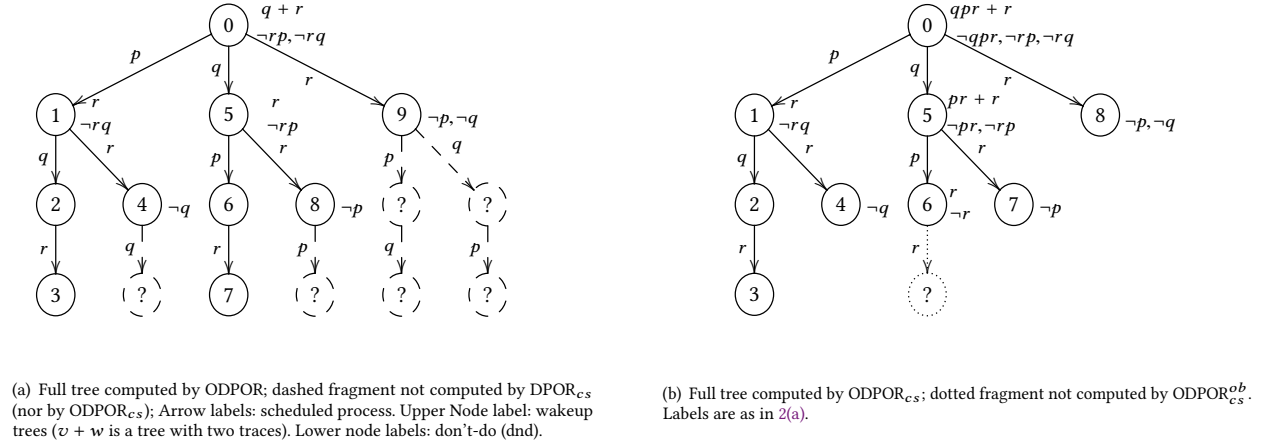
Figure 2: Execution trees computed by DPOR algorithms for our running example starting from x=0
