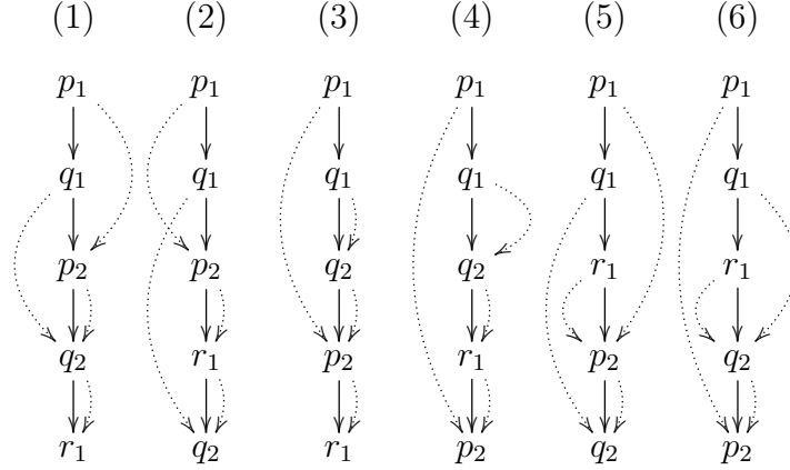
Figure 1.1: Happens-before relations for Example 1
