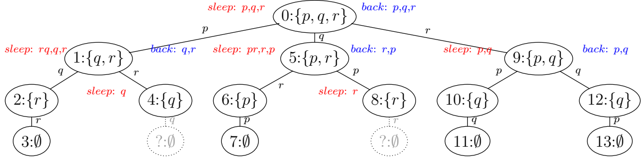
Figure 2.1: Full execution tree computed by \text{DPOR}_{cs} for Example 8; dotted fragment not computed thanks to sleep sets; Arrow labels: scheduled process. Node labels right (in blue): backtrack set (only indicated for nodes with more than one process). Node labels left (in red): sleep set (only indicated for nodes with more than one sequence and sequences propagated from their parents).
