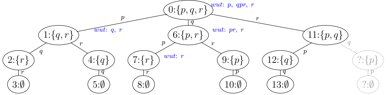
Figure 2.2: Full execution tree computed by \text{ODPOR}^{ob} for Example 9; dotted fragment not computed thanks to the notion of observability; Arrow labels: scheduled process. Node labels right (in blue): wake-up tree (only indicated for nodes with more than one sequence and sequences propagated down).
