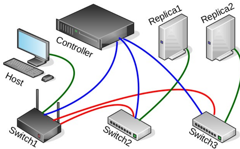
Figure 4.1: Structure of the SDN load-balancer in Example 18.
