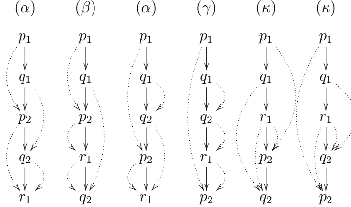
Figure 1.3: Happens-before relations for Example 6
