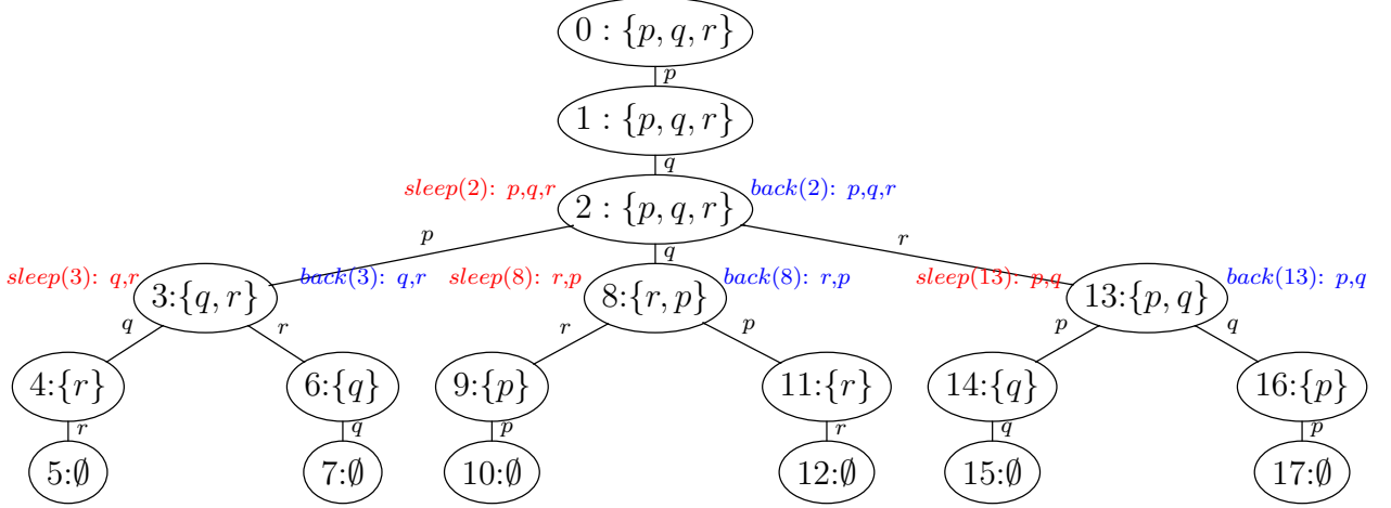
Figure 1.2: Full execution tree computed by DPOR for Example 5. Node labels: Enabled Processes. Arrow labels: scheduled process. Node labels right (in blue): backtrack set. Node labels left (in red): sleep set. Both backtrack and sleep sets are only indicated for nodes with more than one process.
