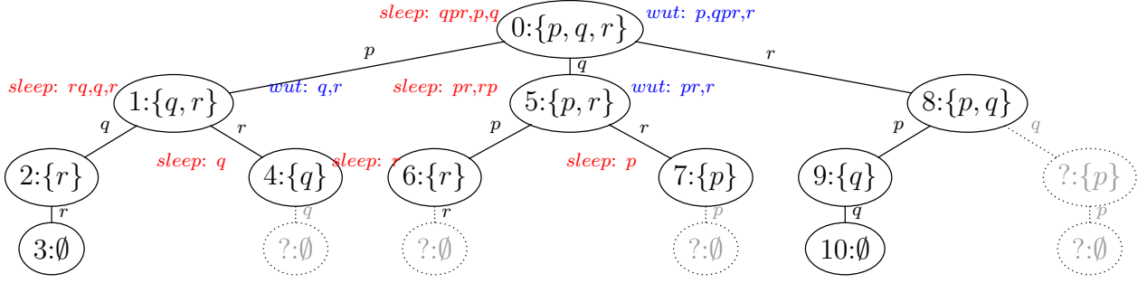
Figure 2.3: Full execution tree computed by ODPOR_{cs}^{ob} for Example 10; dotted fragment not computed thanks to sleep sets; Arrow labels: scheduled process. Node labels right (in blue): wake-up tree (only indicated for nodes with more than one sequence). Node labels left (in red): sleep set (only indicated for nodes with more than one sequence and sequences propagated from their parents).
