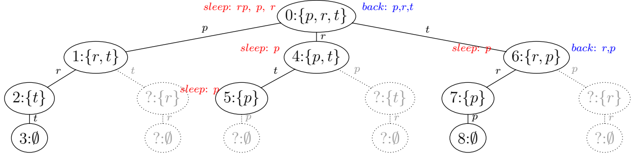
Figure 3.1: Full execution tree computed by CDPOR for Example 17; Arrow labels: scheduled process. Node labels right (in blue): backtrack set (only indicated for nodes with more than one process). Node labels left (in red): sleep set (only indicated for nodes with more than one sequence and sequences propagated from their parents).
