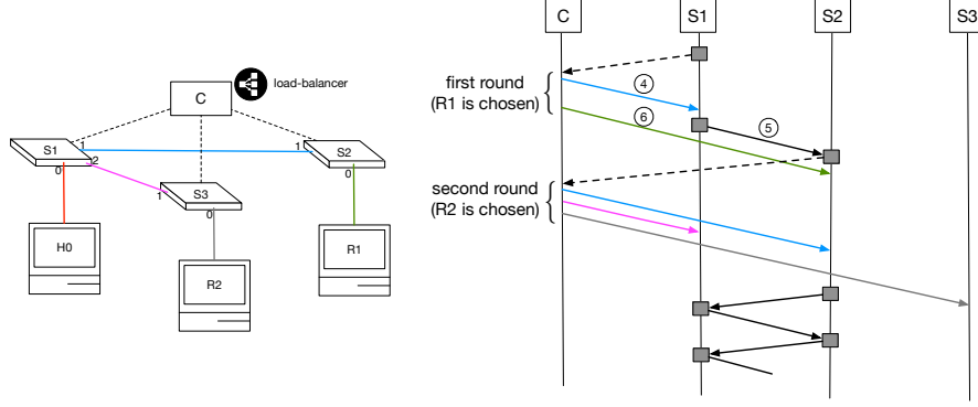
Figure 1: Example SDN load-balancer. On the left: structure of the SDN. On the right: messages exchanged in a possible execution of a naive controller program. Coloured arrows stand for control messages to switches, indicating which flow rule to install (colours specify the link to be used for the forwarding). Grey boxes and arrows among them represent packet forwarding. Dashed arrows indicate messages to the controller.
