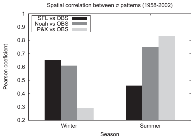
Figure 8: Spatial correlation between simulated and observed patterns of \sigma . Period 1958–2002.
