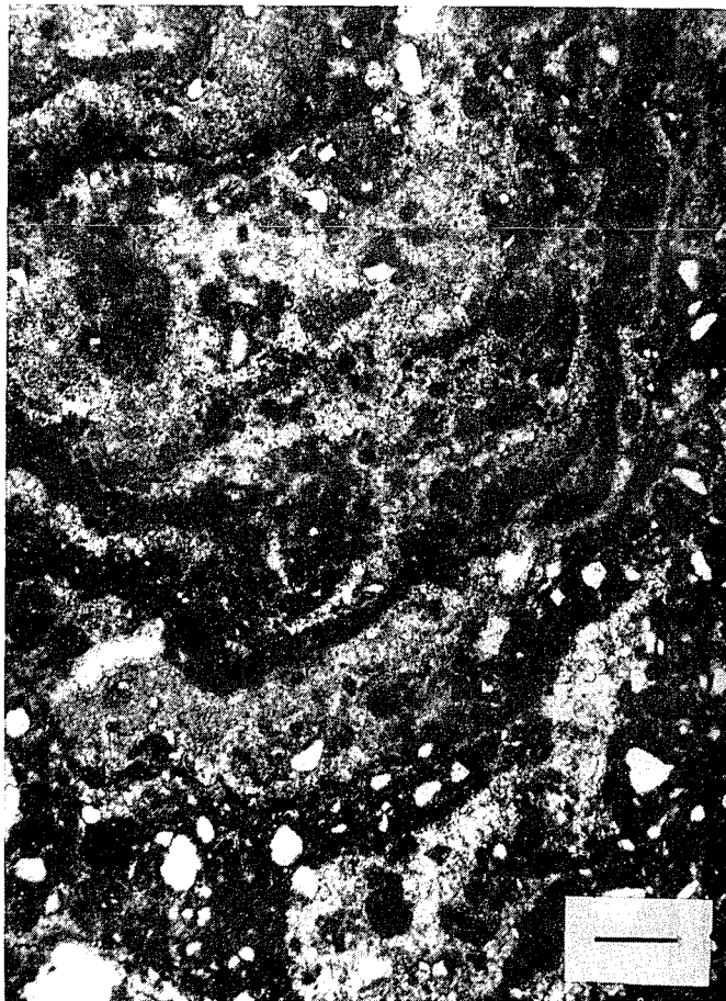
Fig. 11.- Photomicrograph of the layers of the pisolith coatings. Note the alternation of dark dense micrite with scarce silt grains and clearer laminae formed of peloids, terrigenous grains and sparite mosaics. Scale bar represents 200 \mu .
