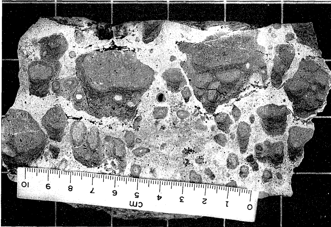
Fig. 10.- Polished hand sample showing a marked development of gravitational pisoliths.
