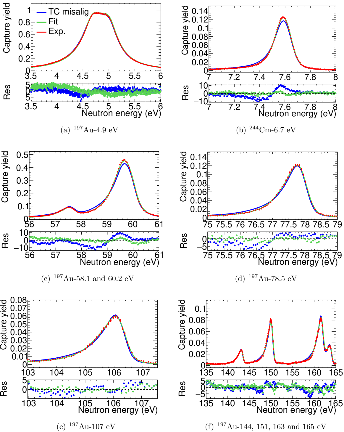
Figure 2.31: Experimental ^{197}\text{Au} and ^{244}\text{Cm} capture yields for a circular sample with 2.5 mm radius compared with two theoretical yields. One uses one of the RF in Figure 2.29 (TC misalig), which is the RF from MC calculations which better reproduces the experimental data, and the other (Fit) uses the RF obtained from the fitting method explained in the body text. In the bottom panel of each figure the residuals are plotted.
