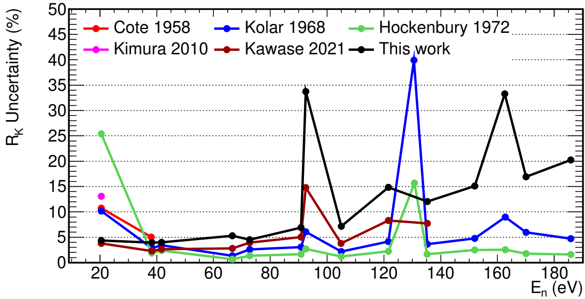
Figure 6.28: Comparison between the uncertainties in the R_K values measured in this work and the data of previous measurements for the resonances of ^{240}\text{Pu} below 200 eV.
