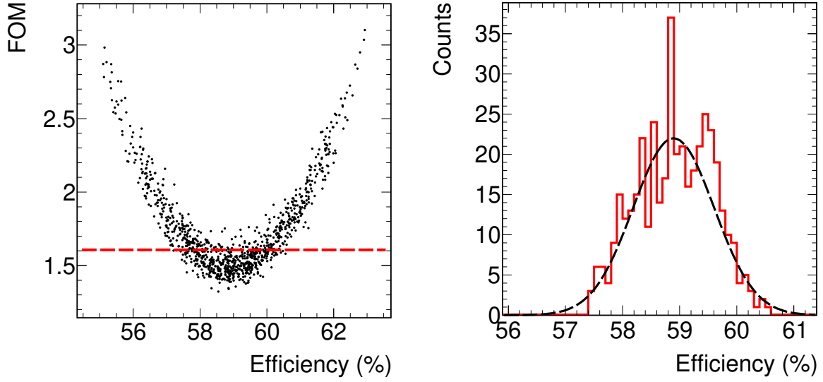
Figure 3.6: FOM and detection efficiency for 2.5 < E_{\text{sum}} (\text{MeV}) < 6 and m_{\text{cr}} > 2 obtained in the simulation of 1000 different ^{244}\text{Cm}(n,\gamma) cascades. On the left panel, a scatter plot of the two values. On the right panel, the values of the efficiency with a FOM < 1.6 are histogrammed and fitted with a Gaussian function.
