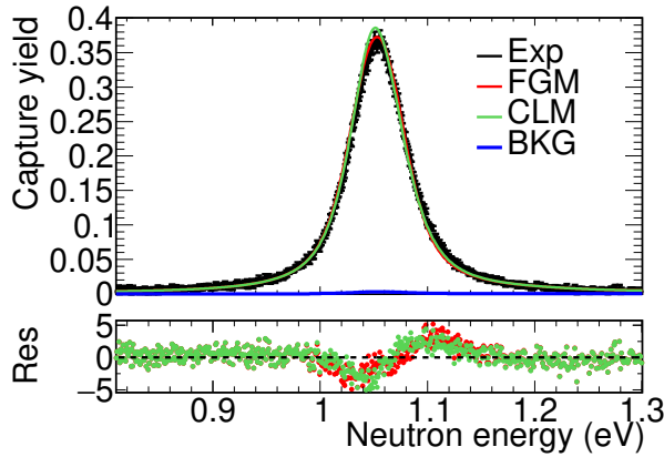
Figure 6.2: Experimental capture yields (Exp) in the energy range of the strongest ^{240}\text{Pu} resonance compared to the yield obtained with the JEFF-3.3 RP using two Doppler models: the FGM (FGM) and the CLM (CLM). The background (BKG) in the resonance is very small.
