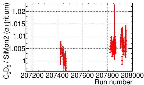
Figure 2.18: Ratio (re-scaled) between the number of counts in C_6D_6 and the SiMon2 for each run measuring the ^{244}Cm sample in EAR2 for primary pulses.
