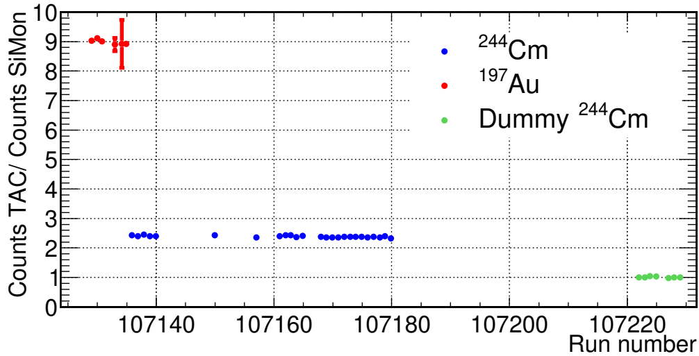
Figure 4.11: Number of events in the TAC with 2.5 < E_{\text{sum}} \text{ (MeV)} < 6 cuts divided by the number of counts in the SiMon detector, for each run with beam. All the ratios have been normalised to the value obtained for run 107222.
