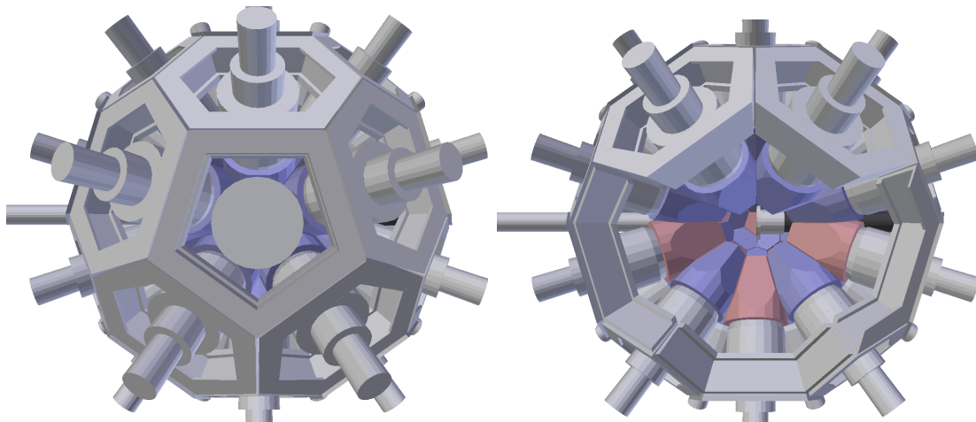
Figure 4.12: View of the TAC as implemented in Geant4 used for the Monte Carlo simulations. The left panel shows all the TAC modules, and the right panel shows the detector removing some modules to see the centre of the TAC.
