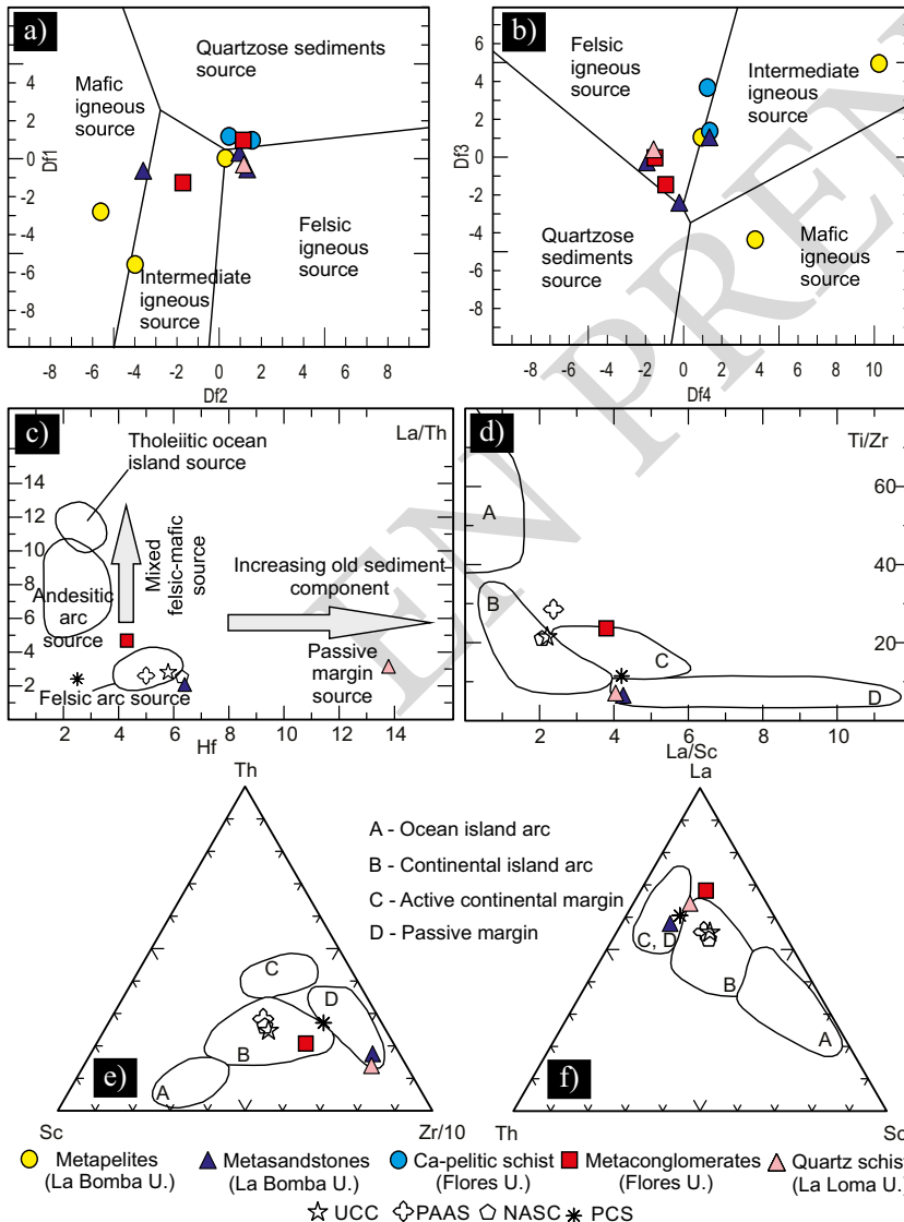
Figure 16. Source areas and tectonic setting diagrams. a) and b) Roser and Korsch, (1988). Discriminant function (Df) calculated as: Df1 = 56.500 \text{ TiO}_2/\text{Al}_2\text{O}_3 - 10.879 \text{ Fe}_2\text{O}_3/\text{Al}_2\text{O}_3 + 30.875 \text{ MgO}/\text{Al}_2\text{O}_3 - 5.404 \text{ Na}_2\text{O}/\text{Al}_2\text{O}_3 + 11.112 \text{ K}_2\text{O}/\text{Al}_2\text{O}_3 - 3.89 ; Df2 = 30.638 \text{ TiO}_2/\text{Al}_2\text{O}_3 - 12.541 \text{ Fe}_2\text{O}_3/\text{Al}_2\text{O}_3 + 7.329 \text{ MgO}/\text{Al}_2\text{O}_3 + 12.031 \text{ Na}_2\text{O}/\text{Al}_2\text{O}_3 + 35.402 \text{ K}_2\text{O}/\text{Al}_2\text{O}_3 - 6.382 ; Df3 = 0.445 \text{ TiO}_2 + 0.070 \text{ Al}_2\text{O}_3 - 0.250 \text{ Fe}_2\text{O}_3 - 1.142 \text{ MgO} + 0.438 \text{ CaO} + 1.475 \text{ Na}_2\text{O} + 1.426 \text{ K}_2\text{O} - 6.861 ; Df4 = -1.773 \text{ TiO}_2 + 0.607 \text{ Al}_2\text{O}_3 + 0.760 \text{ Fe}_2\text{O}_3 - 1.500 \text{ MgO} + 0.616 \text{ CaO} + 0.509 \text{ Na}_2\text{O} - 1.224 \text{ K}_2\text{O} - 9.090 . In all discriminant functions \text{Fe}_2\text{O}_3 represents total Fe content. c) Floyd and Leveridge (1987). d) - f) Bhatia and Crook (1986).
