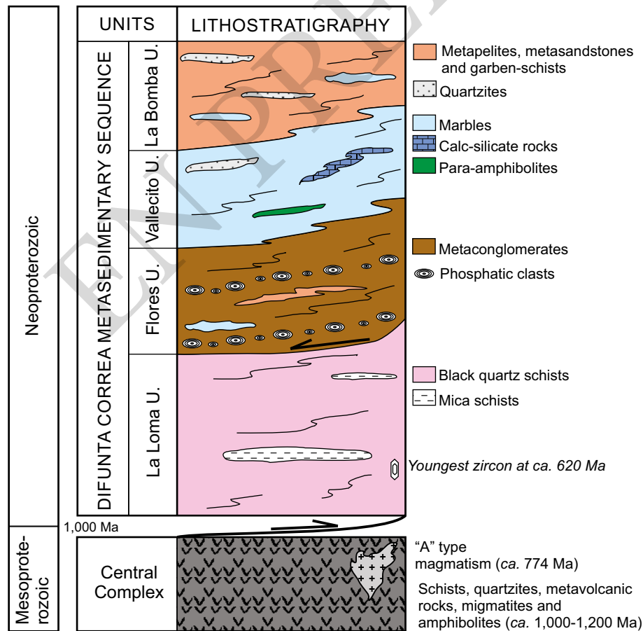
Figure 4. Schematic lithostratigraphic column of the DCMS. The youngest zircon age is from Rapela et al. (2005, 2015)
