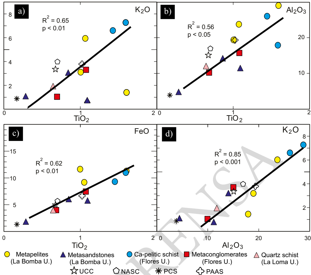
Figure 13. Variation plots of major elements against TiO_2 and Al_2O_3 . Values in weight percent. a) Sample PPL-424 was not considered in correlation coefficients. b) - d) Sample SPP-22013 was not considered in correlation coefficients due to their carbonaceous cement.
