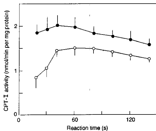
FIG. 2. Effect of AICAR on CPT-I activity at different reaction times. Hepatocytes were preincubated for 15 min in the absence (○) or in the presence (●) of 0.5 mM AICAR. Subsequently, aliquots were removed to determine CPT-I activity at different reaction times by method A. Note that enzyme velocity (and not product accumulation) is represented on the y-axis. Results correspond to six different hepatocyte preparations.
