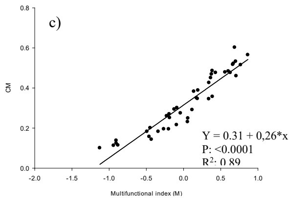
Figure S3. Relationships between our multifunctionality index based on the average of Z-scores of ecosystem functions and other multifunctionality indices: a) the average of multiple functions, previously standardized by dividing by the maximum (SD, Mouillot et al. , 2011); b) this average minus the standard deviation (SDSE, Pasari et al. , 2011); and (c) the cross-multiplied ten soil variables previously standardized by dividing by the maximum (CM, Bowker et al. , 2013).
