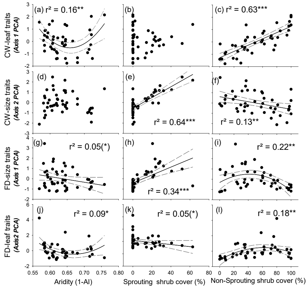
Figure S4. Responses to aridity (1- aridity index [precipitation/potential evapotranspiration]) and shrub encroachment of community weighed traits (CWT) and functional diversity (FD) evaluated with leaf and size related traits. Co-variations among traits are shown in Fig. 2 for CWT and FD. Community responses to: aridity (1-Aridity Index [AI]) are shown in panels (a, d, g, j); responses to shrub encroachment separating sprouting shrub and non-sprouting shrub are shown in panels (b, e, h, k) and (c, f, i, l) respectively. The black solid line indicates significant ( P < 0.05 ) relationships; the grey dash lines show 95% confidence intervals in these cases. We provided the R^2 of the linear regression in each panel. (*), P < 0.09 ; *, P < 0.05 ; **, P < 0.01 ; ***, P < 0.001 .
