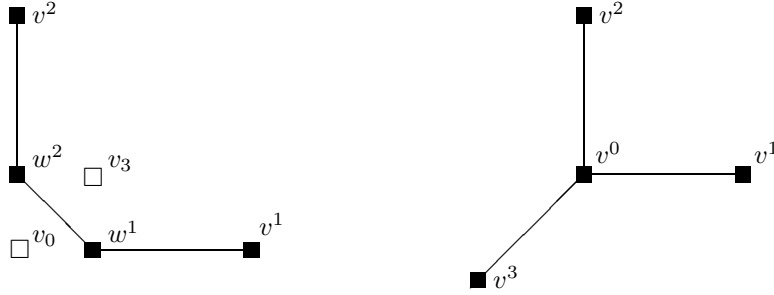
Figure 1: Non-pendant vertices: cases d_3 < 0 and d_3 > 0 .
