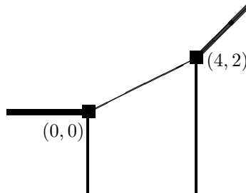
Figure 3: A weighted tree \mathcal{C} in Z = 0 .
