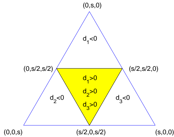
Figure 2: Section of octant \mathcal{O} given by s_{21}^+ + s_{32}^+ + s_{31}^+ = s .
