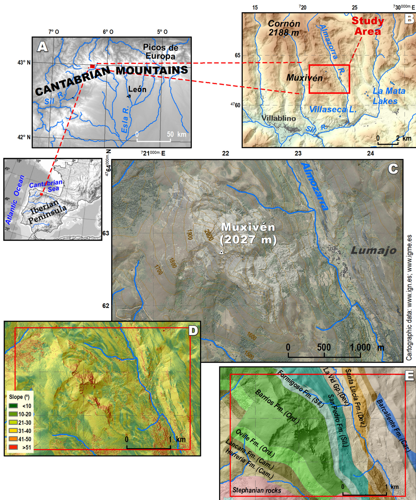
Fig. 1. Location of the study area within the Iberian Peninsula and the Cantabrian Mountains (A), and the upper Sil River Basin (B). Orthophoto and topographical map (C), together with the slope (D) and geological and lithological conditions (E) existing in the area. Cam: Cambrian, Ord: Ordovician, Sil: Silurian, Dev: Devonian, Car: Carboniferous.
