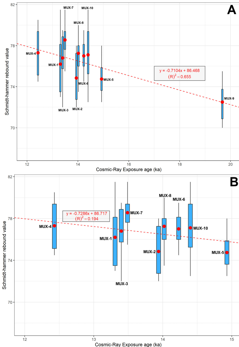
Fig. 9. Correlation between mean SH-R values and ^{10}\text{Be} CRE ages. A: all samples included. B: all samples except MUX-9 included.
