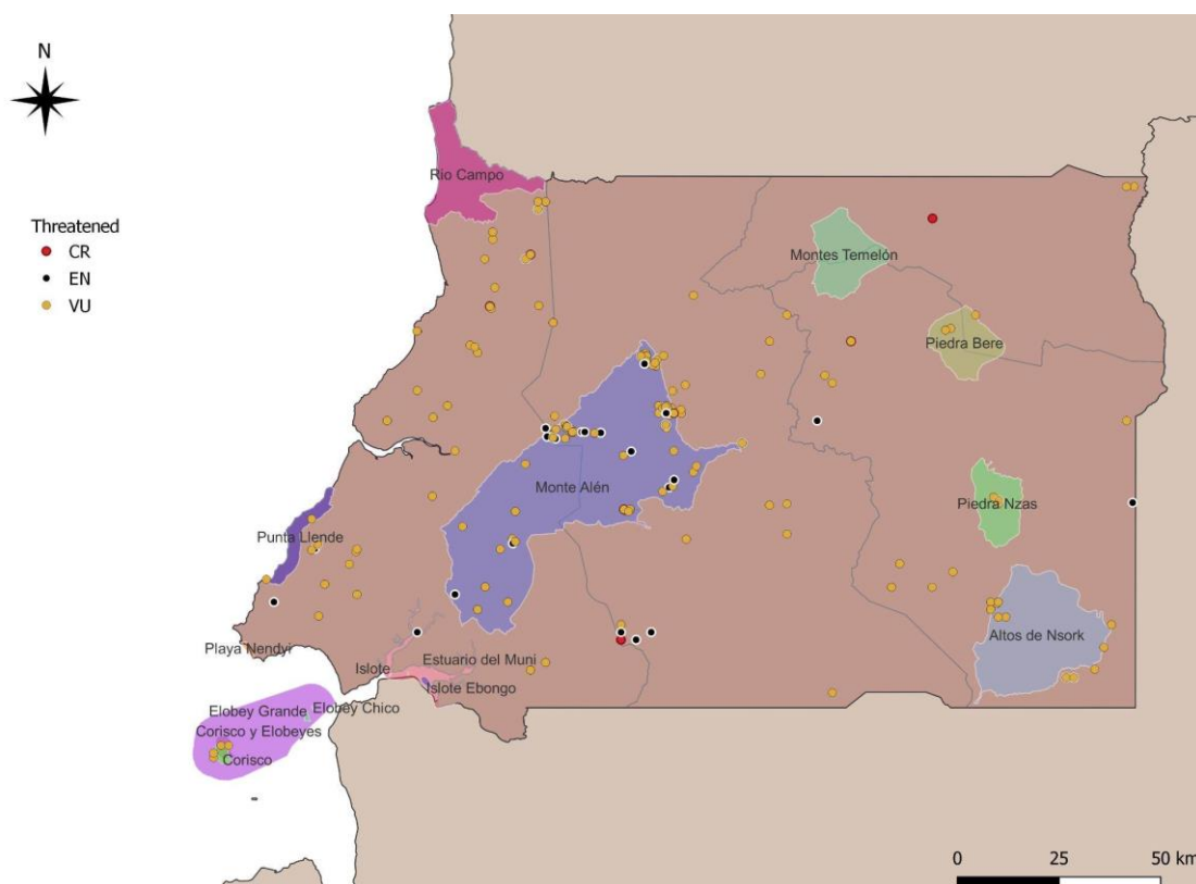
Fig. 17. Protected Areas of Río Muni. Dots indicate the occurrences of threatened species: CR (red), EN (black), VU (yellow).
