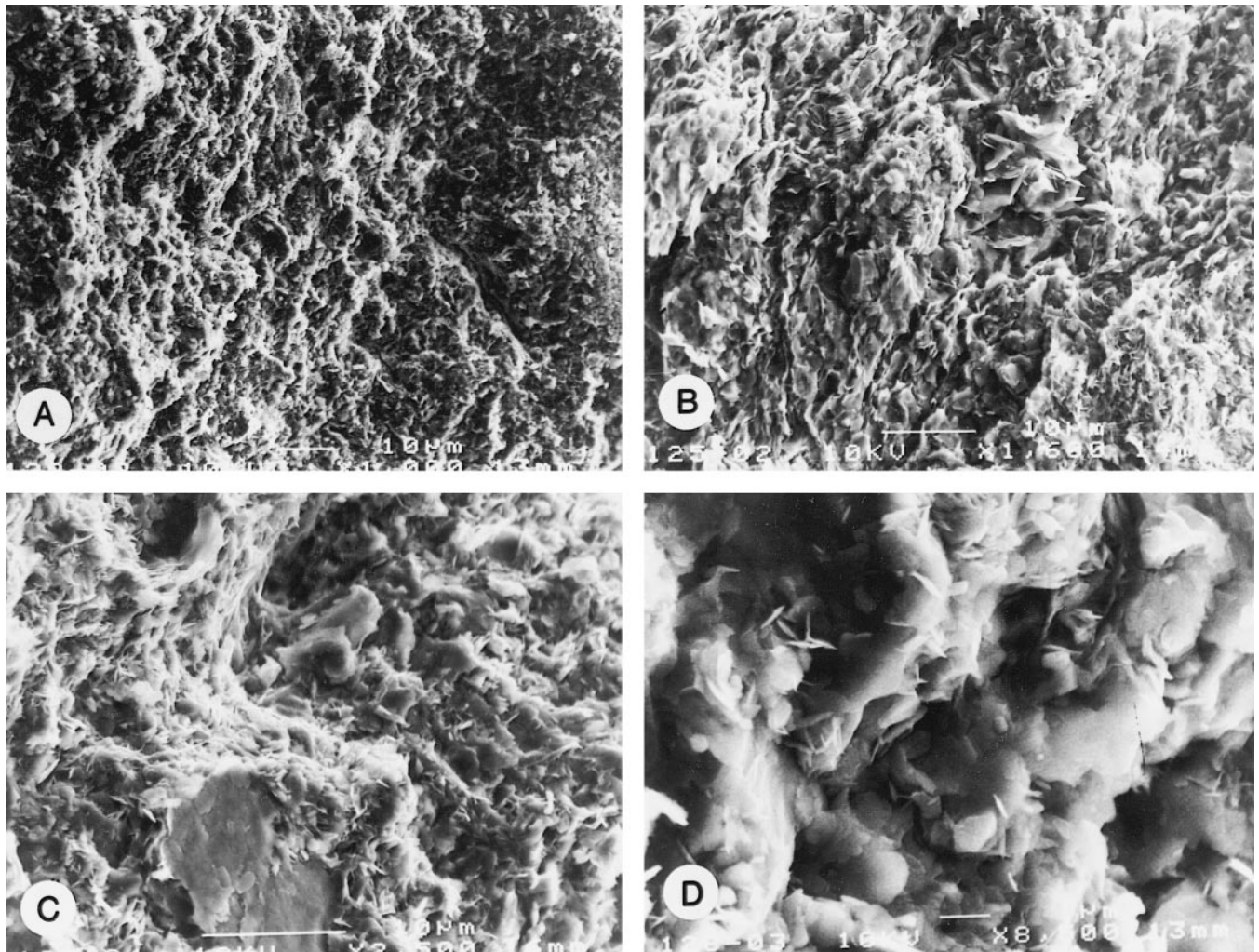
FIG. 9.—Scanning electron micrographs of silt infiltration structures (siltans) and clay skins (argillans) of paleosols in the Lashly Formation, Antarctica: A ) siltan of coated grains; B ) narrow skin of coarse clay; C ) laminated clay skins; D ) illitic clay of matrix. Specimen number for B is R1838. Others are from R1841.
