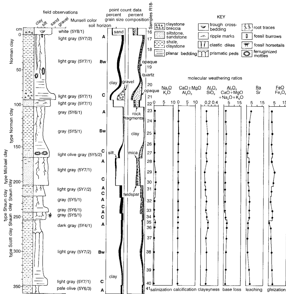
FIG. 8.—Measured section, Munsell colors, soil horizons, grain size, mineral composition, and selected molecular weathering ratios of the type Norman, Michael, Shaun, and Scott pedotypes and other paleosols from 258–263 m in the measured section (Fig. 2) in the Allan Hills, Antarctica.
