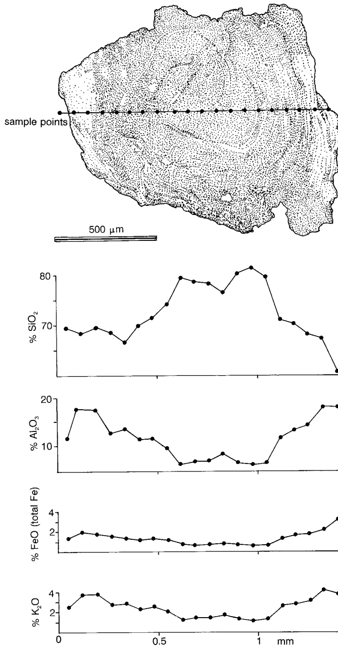
FIG. 6.—Microprobe traverse of white root trace from the Lashly Formation, Antarctica, showing concentric interlamination of chalcedony and illite (Specimen R1841).
