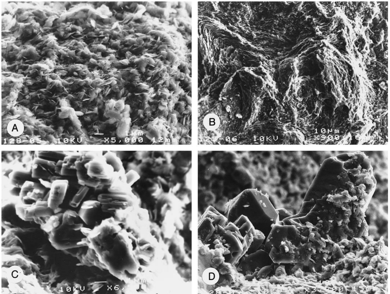
FIG. 4.—Scanning electron micrographs of minerals in white root traces of the Lashly Formation, Antarctica: A ) clay-encrusted chalcedony fibers; B ) chalcedony (massive) and clay (laminated); C ) sanidine in volcanic rock fragment; D ) orthoclase in volcanic rock fragment. Specimen numbers are R1838 (C) and R1841 (others).
