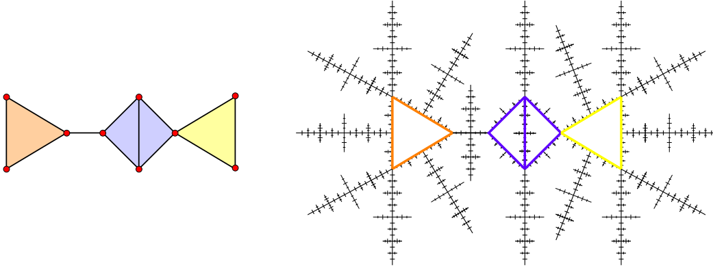
FIGURE 12. The dual graph associated to a good resolution \pi of a normal surface singularity X , with bricks shaded, and its associated space \mathcal{V}_X of normalized semivaluations.
