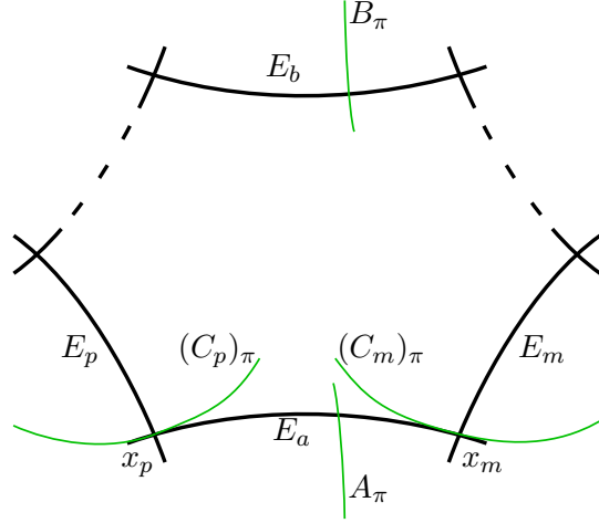
FIGURE 9. Geometric situation of Proposition 1.45.
