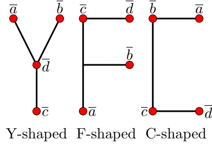
FIGURE 7. The Y -shaped, F -shaped and C -shaped trees in the proof of Theorem 1.38.
