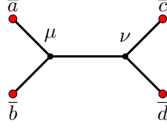
FIGURE 5. The case of an H -shaped tree in the proof of Theorem 1.38 .
