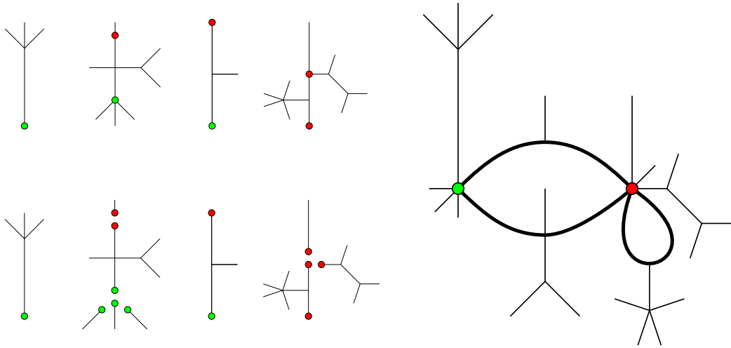
FIGURE 10. A graph of \mathbb{R} -trees, its regularization, their realization and the corresponding skeleton.
