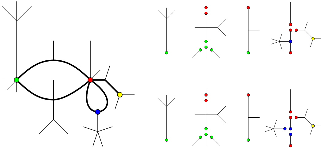
FIGURE 11. Refinement of a graph of \mathbb{R} -trees.
