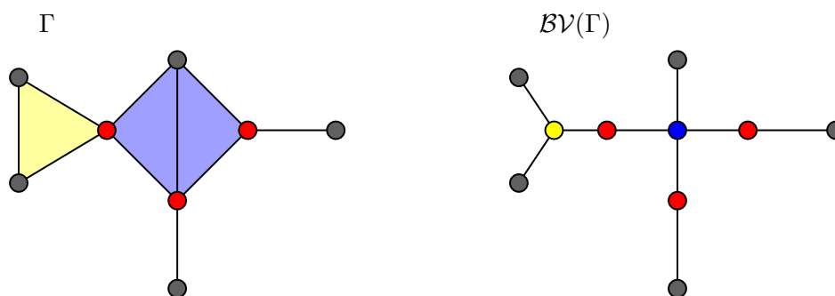
FIGURE 4. The brick-vertex tree of a connected graph.
