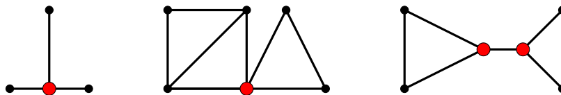
FIGURE 3. A few separable graphs and their cut-vertices marked in red.
