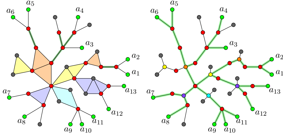
FIGURE 8. Example 1.39, in which the hypothesis of Theorem 1.38 about valencies of bricks is satisfied.
