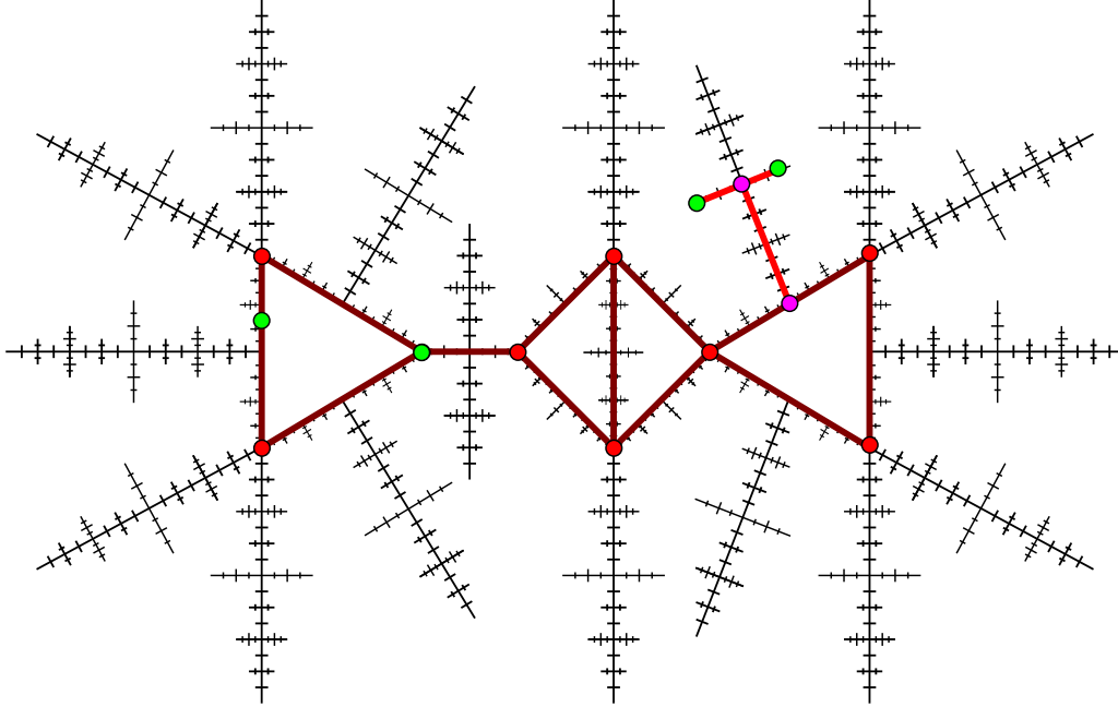
FIGURE 14. Graphs embedded in \mathcal{V}_X , illustrating the proof of Theorem 2.53 .
