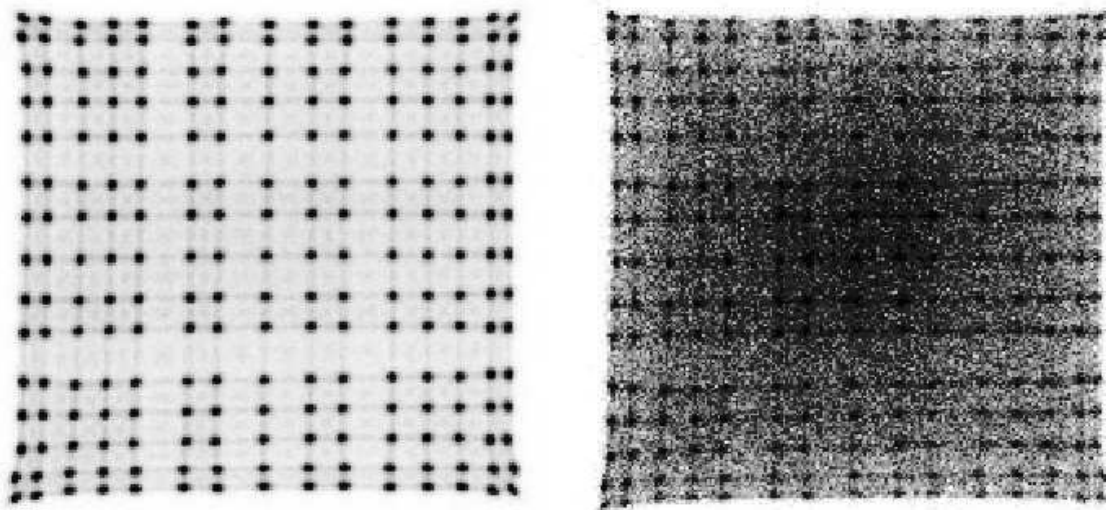
Figure 1.11. Simulated flood histogram for a Hamamatsu 8520-C12 coupled to an array of 15 × 15 LYSO crystals with (right, activity = 1mCi) and without (left, activity = 10 µCi) pile-up events. Pile-up produces mispositioned of detected photons.
