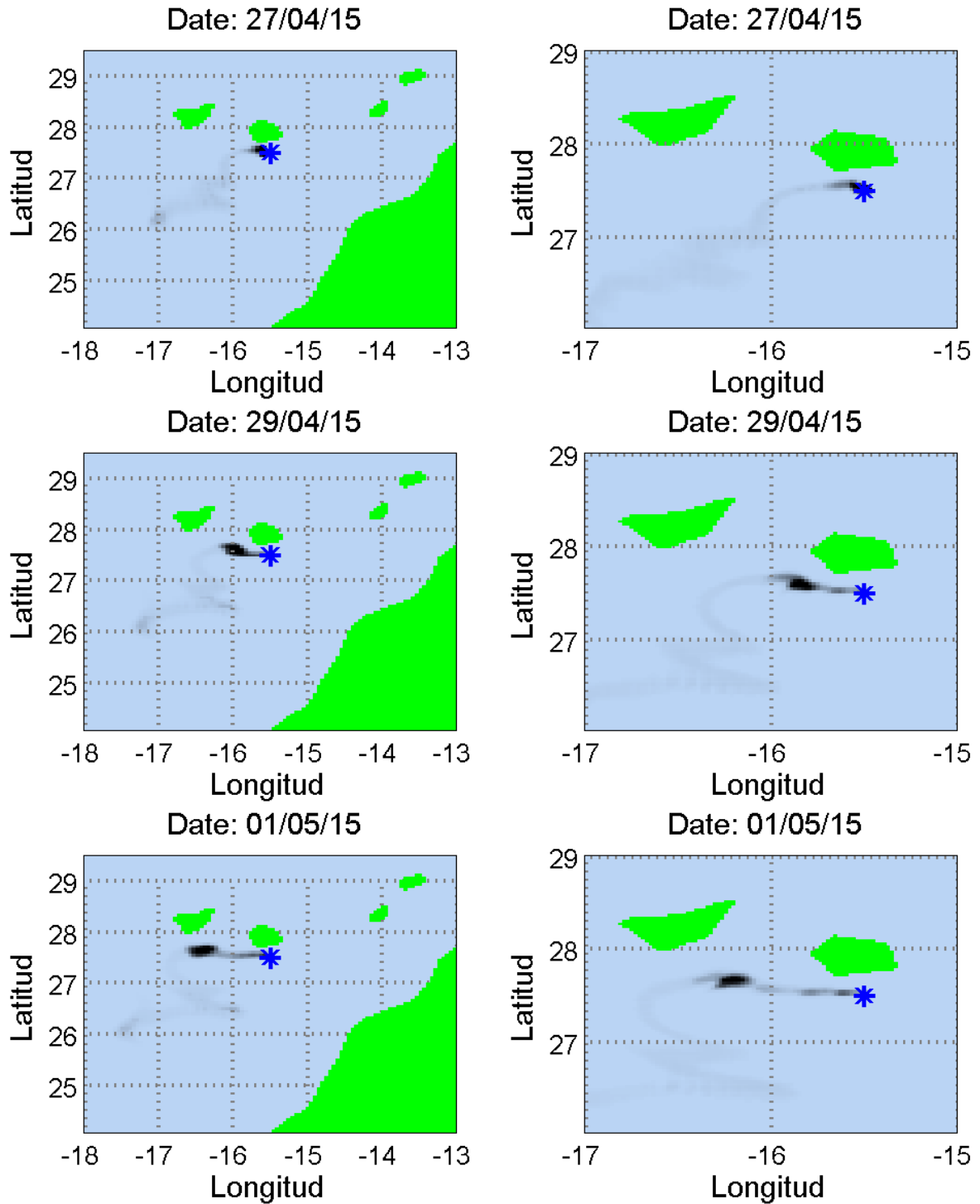
Figure 5: Oil concentration simulated by the model, considering the computational domains ( Left ) \Omega and ( Right ) \Omega_z , presented in this work for the dates: ( Top ) April, 27 2015, ( Middle ) April, 29 2015 and ( Bottom ) May, 01 2015. The coast is also represented in green. The position of the Oleg Noydenov ship is presented by a blue star.
