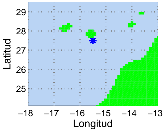
Figure 3: Computational domain \Omega considered for the numerical experiments presented in Section 3. The land is presented in green. The position of the Oleg Naydenov ship is presented by a blue star.
