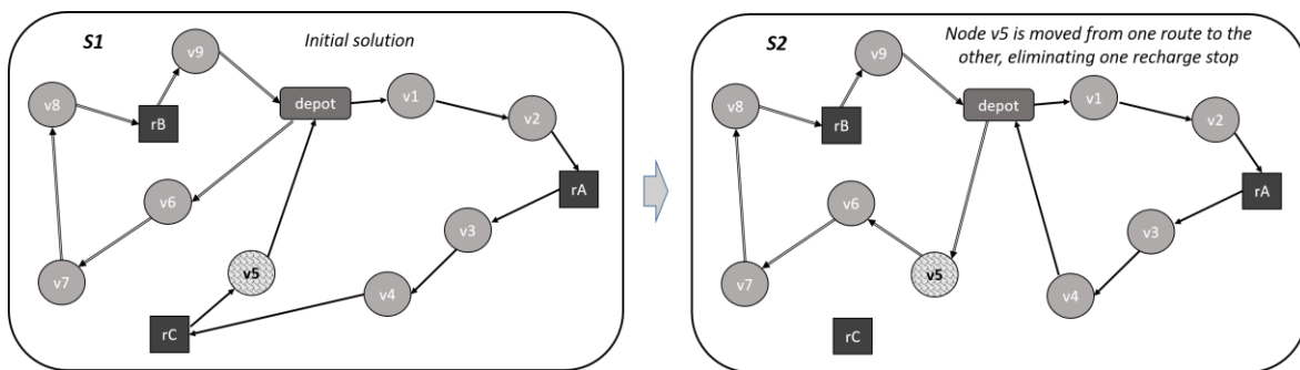
Figure 3: Illustration of the Reinsertion operator
