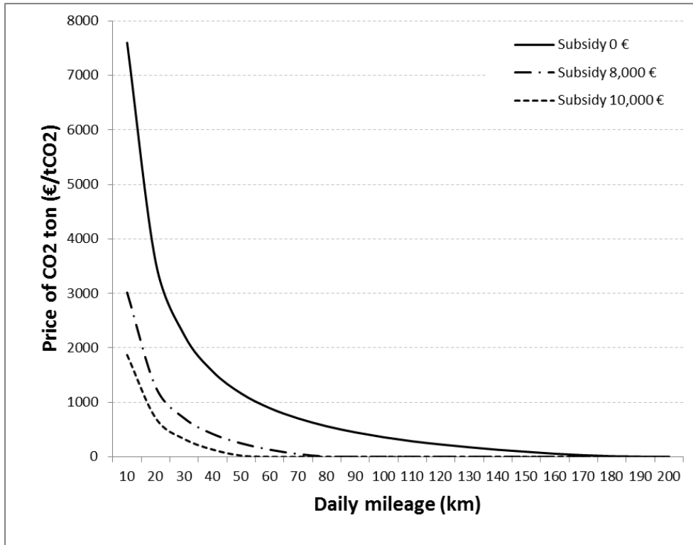
Figure 3: CO 2 price required to make BEVs competitive as a function of daily mileage, calculated for different subsidy levels
