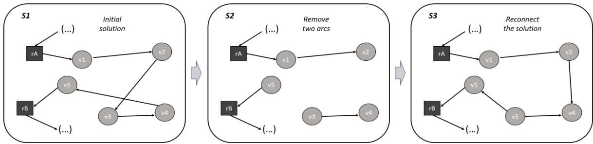
Figure 2: Illustration of the 2-Opt operator
