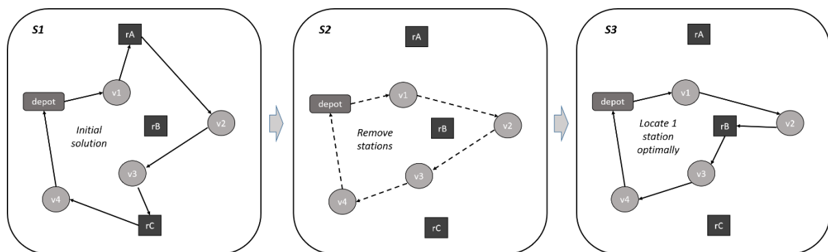
Figure 1: Illustration of the Recharge Relocation operator
