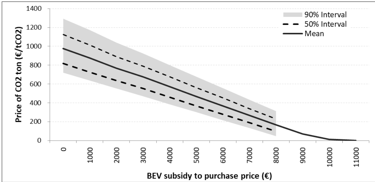
Figure 2: CO 2 price that makes BEVs competitive for different subsidy levels
