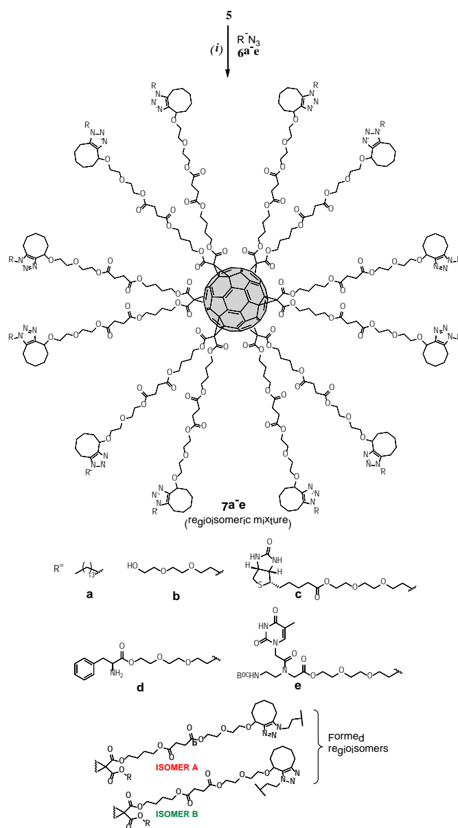
Scheme 1 Synthesis of compound 5. Reagents and conditions: (i) C 60 , DBU, CBr 4 , ODCB, rt, 72h (50%); (ii) H 2 , Pd-C, DCM/MeOH, rt, overnight (100%); (iii) DPTS, DCC, DCM/DMF, rt, overnight (99%).
