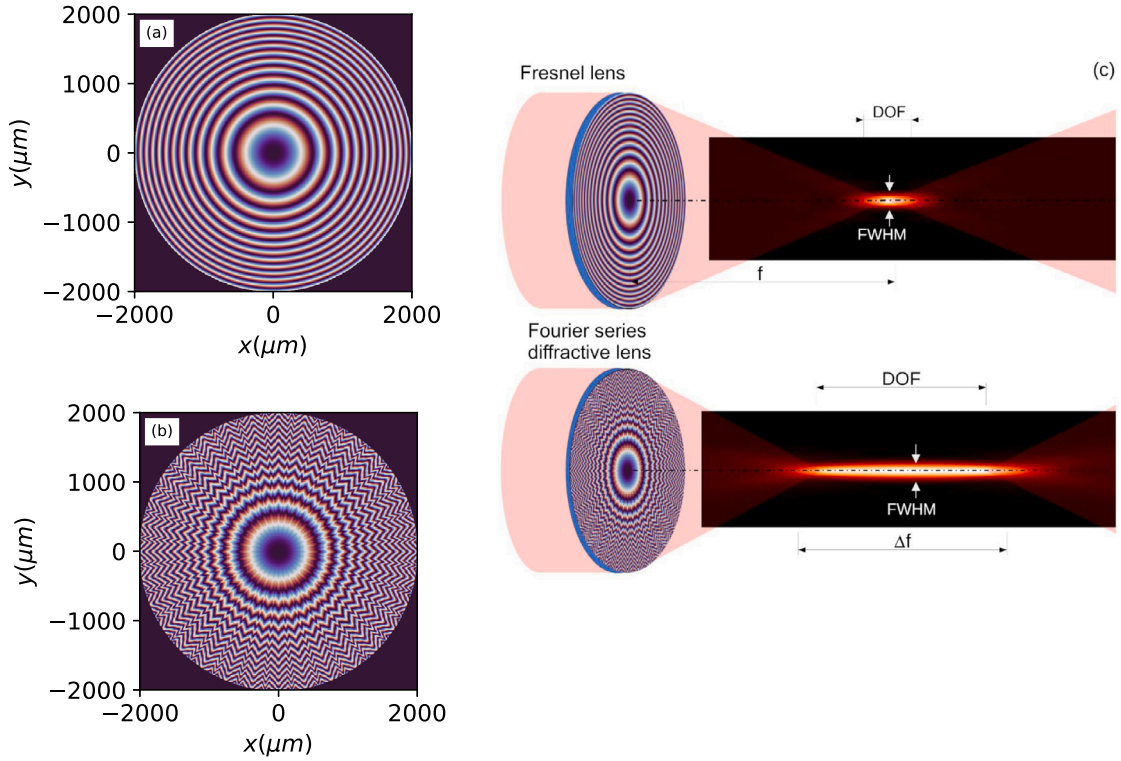
Fig. 1. Phase maps of (a) Fresnel and (b) FSDL lens with D = 4 mm and f' = 250 mm. The FSDL presents a depth of focus \Delta f = 25 mm and 5 Fourier coefficients: a_l = [0.9, 0.7, -0.2, 0.3, -0.1] . (c) Optical scheme for the Fresnel lens and the FSDL, including the expected results for extended depth of focus. The intensity distribution for the FSDL is obtained with coefficients of Table 1a.
