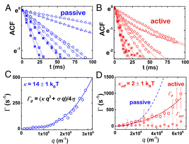
Fig. 5. Time correlation function and relaxation dynamics. Experimental ACFs of a D-F 1 F 0 -GUV in the (A) passive and (B) active cases for azimuthal wave vectors 2 \leq l \leq 10 . Solid lines correspond to fits of the experimental data to Eq. 5. Only the thermal contribution of Eq. 5 was necessary under passive conditions, whereas the bimodal function of Eq. 5 was required for active D-F 1 F 0 -GUVs. Relaxation rates of a D-F 1 F 0 -GUV in the (C) passive and (D) active cases. Thermal frequencies, \Gamma_0 , were fitted using Eq. S8 with \eta = 1 cP (solid lines). For comparison, dashed line in D corresponds to the thermal rate shown in C. \Gamma_{act} is the characteristic rate of the metabolic active mode.
