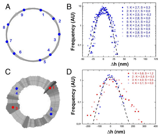
Fig. 3. Mechanical hot-spots of D-F 1 F 0 -GUVs. (A) Fluctuation map of passive D-F 1 F 0 -GUV from B ( t = Ht + 12 min). Points indicate the membrane positions where the PDF is calculated in B. (B) PDF at different points highlighted in A. Dashed line represents the ensemble-averaged PDF as calculated for all contour points of the vesicle. (C) Active D-F 1 F 0 -GUV from A ( t = Ht + 12 min). Points indicate membrane positions where the PDF is calculated in D. (D) PDF at different points highlighted in C. Dashed line represents the ensemble-averaged PDF as calculated for all points of the vesicle. PDFs from points 1 and 3 deviate from Gaussianity. Note that B and D have different scales to highlight the probable out-of-equilibrium signature of hot spots.
