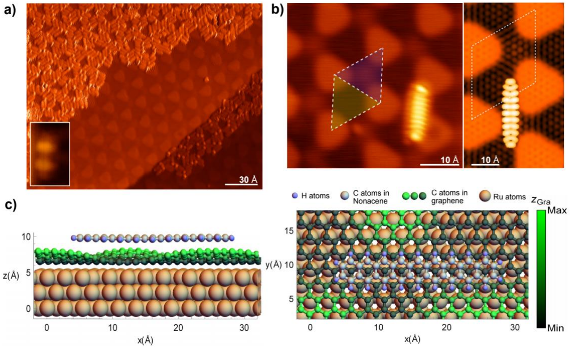
Fig. 2 (a) STM topography ( V_b = 1.5 V, I_t = 50 pA) image of a-bisdiketone nonacene precursors on gr/Ru(0001) after room temperature deposition, recorded at 4.6K. The a-bisdiketone nonacene precursors self-assemble by avoiding the ripples of the moiré pattern. Inset shows a topographic image of a single a-bisdiketone nonacene precursor. The two bright protrusions are assigned to the a-diketone groups pointing upwards. (b) Left panel: STM image ( V_b = 1.7 V, I_t = 100 pA) of a nonacene molecule adsorbed on the gr/Ru(0001) surface after being exposed to visible light ( \lambda = 470 nm) for 90 minutes. The right panel shows the simulated STM image. (c) DFT calculated geometry showing the most stable physisorbed configuration of a nonacene molecule on gr/Ru(0001). The left panel shows the lateral view and the right panel the top view. Color coding as indicated in the figure legend.
