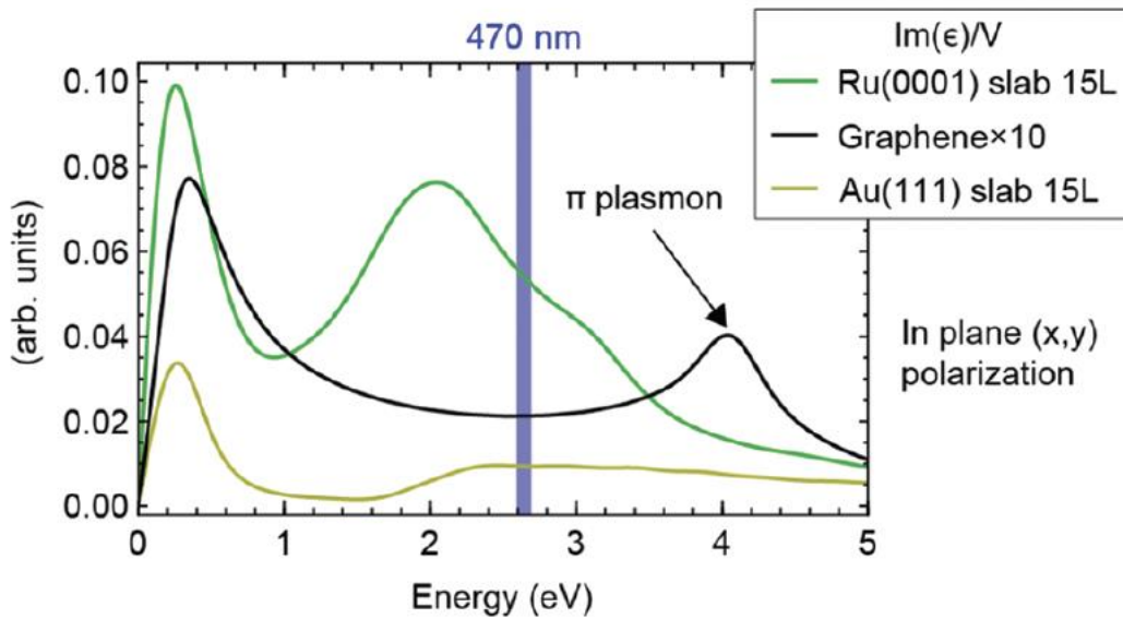
Fig.4: Imaginary part of the dielectric function, \epsilon_2(\omega) = Im[\epsilon(\omega)] , per unit volume, representing the optical properties of the three analyzed materials, as obtained in a Linear Response TD-DFT calculation. The graphene results are multiplied by 10 to visualize them on the same scale as Au and Ru. The vertical blue gridline marks the energy position of the light used in the experiment.
