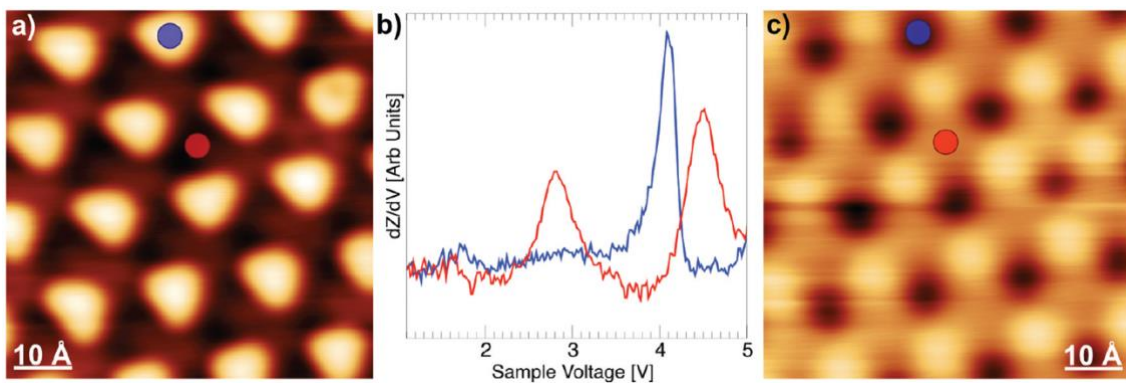
Fig 3 (a) STM topographic image ( 9 \times 9 \text{ nm}^2 , V_b = 0,5 \text{ V} , I_t = 100 \text{ pA} ) measured at 4.6 K. (b) dZ/dV curves measured on the moiré superstructure reflecting the energy position of the corresponding field emission resonances. The blue curve was acquired on the ripples of the moiré (blue dot in panel (a)). The red curve was acquired on the low areas of the moiré (red dot in panel (a)). (c) dZ/dV map measured simultaneously with the image shown in panel (a), showing the spatial distribution of the spectral feature appearing in the red spectrum at +2.85 V in the low areas of the moiré. The coloured dots mark the same positions as in panel (a).
