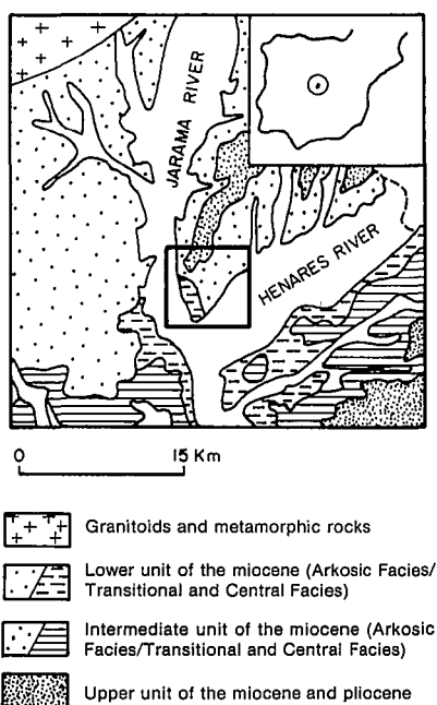
Fig. 1.—Geographic and geologic setting.
