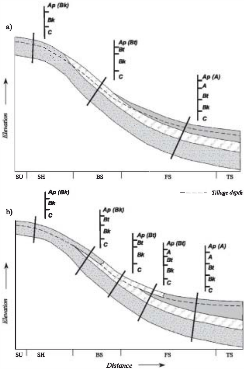
Fig. 3. Idealized model of soil catena modification by tillage. (a) Initial theoretical soil catena; (b) soil catena modified by soil redistribution due to repeated tillage. The genetic horizon material composing the plow layer is shown in parentheses following the Ap symbol. Slope profile elements: SU=summit, SH=shoulder, BS=backslope, FS=footslope, TS=toeslope.
