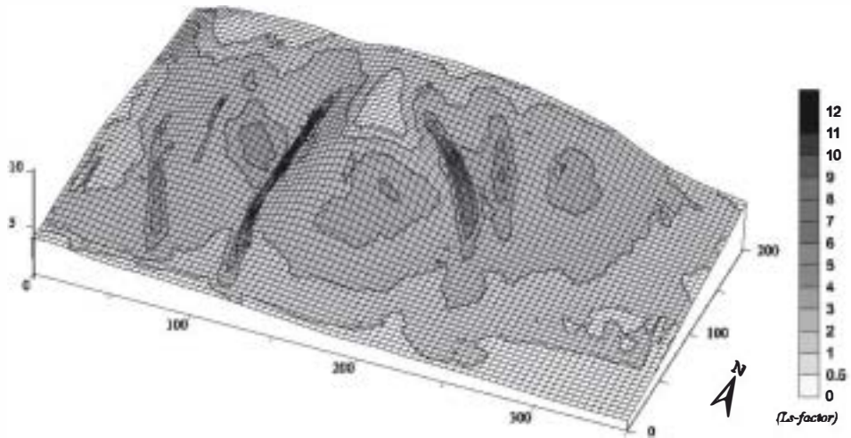
Fig. 12. Spatial variability of the USLE (Universal Soil Loss Equation) topographic LS-factor (slope length and slope gradient factor, dimensionless) in the study site (Axis units in meters).
