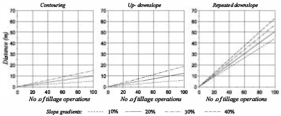
Fig. 14. Nomographs to calculate the distance of expansion of the eroded soil units due to three different patterns of tillage. Tillage downslope is generally the only one possible when the absolute slope gradient is higher than 30%.
