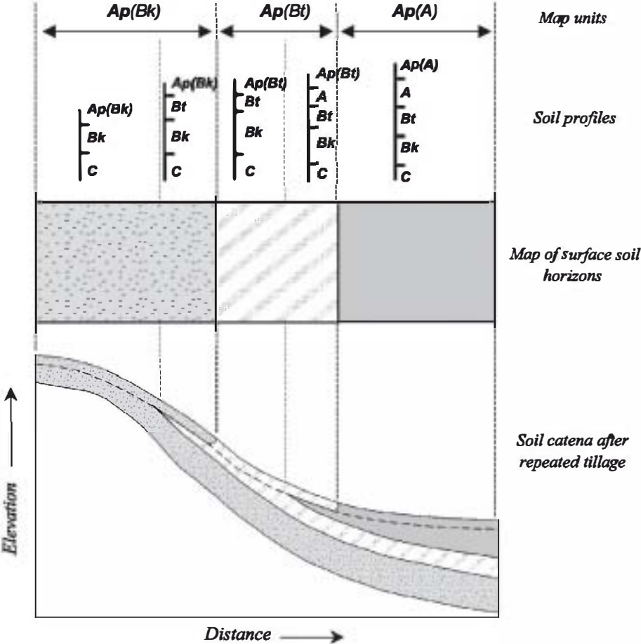
Fig. 13. Increasing variability of soil profiles within map units of surface soil horizons due to soil redistribution by tillage. The genetic horizon material composing the plow layer is shown in parentheses following the Ap symbol.
