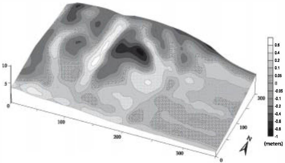
Fig. 8. Simulated soil redistribution by tillage in the study site using the SORET model. Surface elevation changes are given in meters (Axis units in meters).
