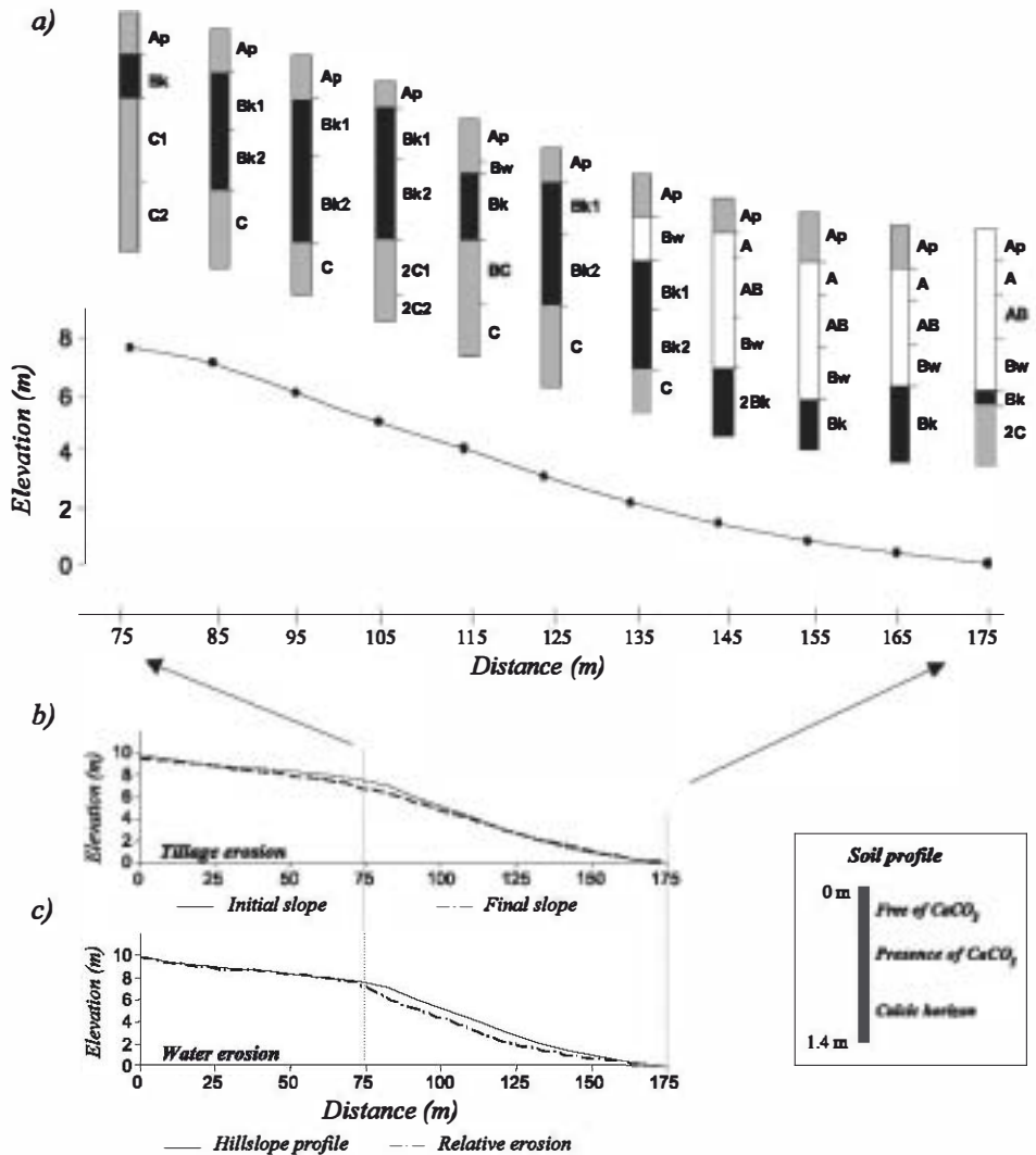
Fig. 10. Spatial variability of soil calcium carbonate (a), predicted soil redistribution by tillage (b), and by water erosion (c) along the Transect 7 (Fig. 5).
