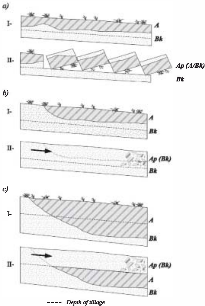
Fig. 2. Modifications of soil profile morphologies due to soil redistribution by tillage. Scheme of processes on three theoretical cases of soil profile: (a) mixing and inversion of the upper soil horizons; (b) substitution of surface soil horizon; (c) partial substitution of the surface soil horizon and formation of a "false truncate soil profile". The genetic horizon material composing the plow layer is shown in parentheses following the Ap symbol (I—before tillage; II—after tillage).
