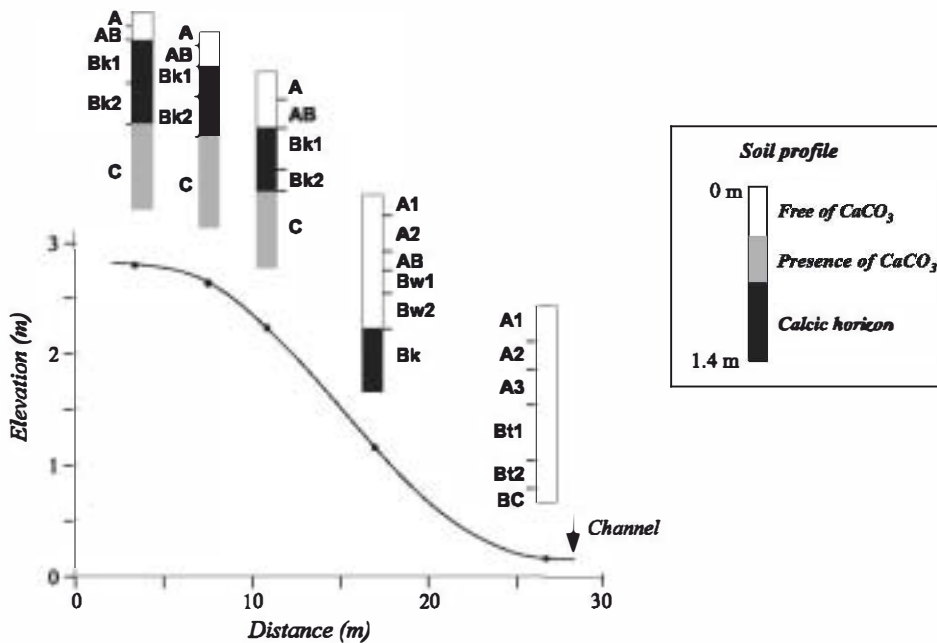
Fig. 7. Spatial variability of soil calcium carbonate in the non-cultivated field.
