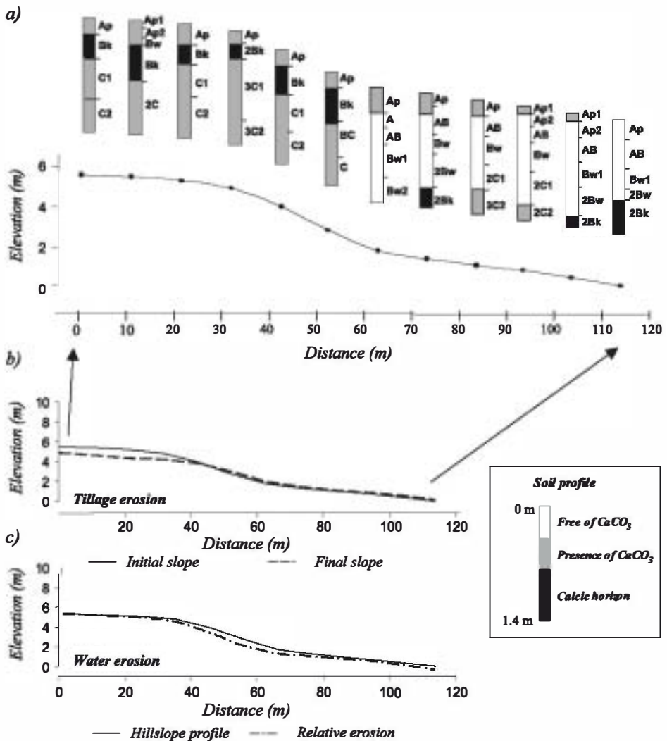
Fig. 9. Spatial variability of soil calcium carbonate (a), predicted soil redistribution by tillage (b), and by water erosion (c) along the Transect 5 (Fig. 5).
