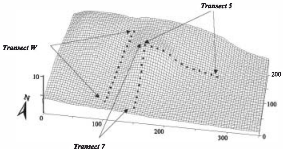
Fig. 5. DTM (Digital Terrain Model) of the study site and localization of soil sampling transects (Axis units in meters).
