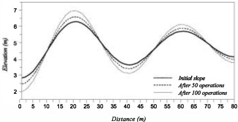
Fig. 1. Simulated long-term effects of soil redistribution by tillage on a theoretical slope profile.
