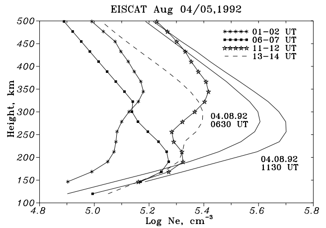
Fig. 7. Observed with EISCAT N e ( h ) profiles for different UT moments of the disturbed day 05 August 1992. Note the modification of normal F2-layer and formation of the layer maximum around 200 km as a reaction to the strong increase in the linear loss coefficient \beta . Quiet time N e ( h ) profiles for 04 August 1992 are shown for a comparison.
