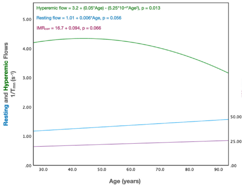
FIGURE 2 Age correlation with Resting and Hyperemic coronary flows and IMR_{Corr} . Regression lines for hyperemic flow (green); resting flow (blue) and IMR_{Corr} (purple). Coronary hyperemic flow starts to significantly decrease after 60 years of age, marking the point in time on which microcirculatory remodeling begins to be functionally evident. On the other hand, both resting flow and IMR_{Corr} progressively increase with age. T_{mn} , mean transit time; IMR_{Corr} , corrected index of microcirculatory resistance. [Color figure can be viewed at wileyonlinelibrary.com ]
