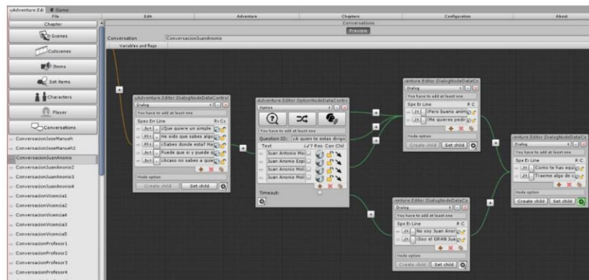
Figure 2. uAdventure's narrative conversation editor
