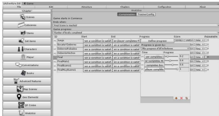
Figure 4. Completables editor in uAdventure’s learning analytics extension, showing a completable’s progress editor open with several completable steps
