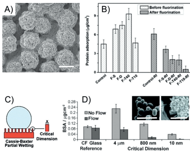
Figure 10. A) SEM image of triple-scaled surfaces (scale bar: 1 \mu\text{m} ). B) Protein adsorption on smooth control, single (-S), dual (-D), and triple scaled (-T10, -T40), corresponding to the size of nanometric silica particles) structured surfaces before and after (-Rf) fluorination. Figure extracted and adapted from Ref. [120a]. C) Sketch of the defined critical dimension to achieve the Cassie–Baxter state. D) Protein adsorption results for fluorocarbon-terminated superhydrophobic surfaces under static and flow conditions. SEM images of micro- and nanometer patterns are shown as insets (scale bars: 10 \mu\text{m} and 800 nm, respectively). Extracted and adapted from Ref. [121].
