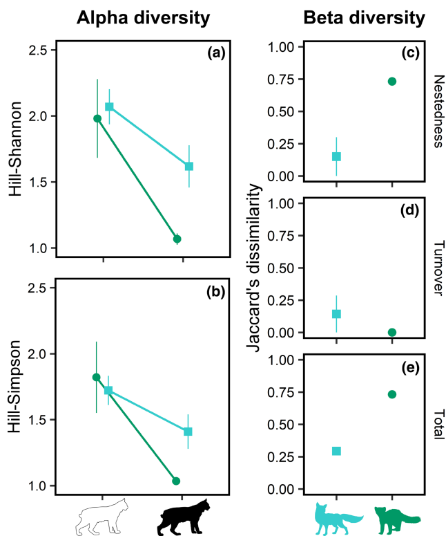
FIGURE 5 Alpha and Beta diversity of dispersed plant species for red fox (blue) and stone marten (green). Alpha diversity is shown in terms of Hill-Shannon (a) and Hill-Simpson (b) indices and was estimated at level of locality and fruiting season. Beta diversity between predation risk scenarios of each fruiting season is expressed in terms of Jaccard's (e) and its components: nestedness (c) and turnover (d). Circles represent observed average values with their correspondent standard errors (bars). Coloured lynx silhouette denotes presence of Iberian lynx and non-coloured silhouette denotes sites without lynx.
